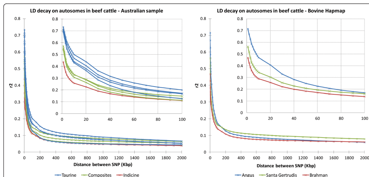
Figure 1 Linkage disequilibrium ( r^2 ) decay on beef cattle autosomes using a selection of Australian cattle breeds and HapMap samples. Additional file 1: Figure S1 discriminates each breed.
