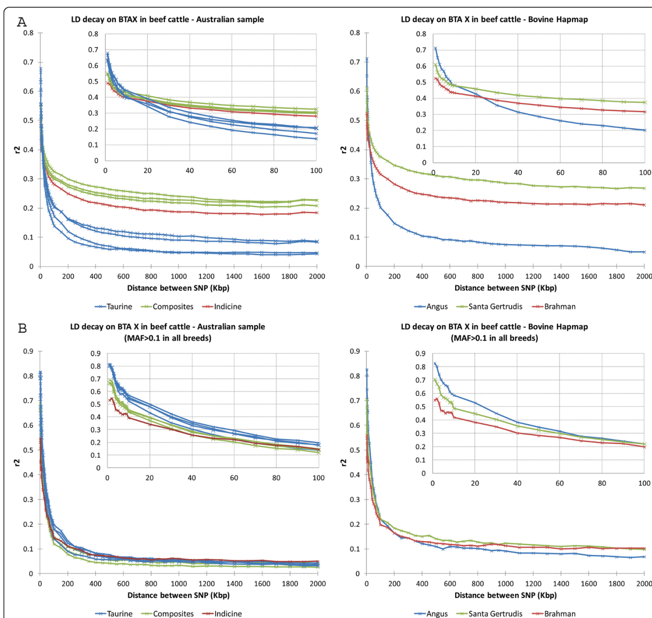
Figure 2 Linkage disequilibrium ( r^2 ) on the X chromosome of beef cattle using all SNPs (A) and only polymorphic SNPs in all breeds (B). MAF = minor allele frequency.
