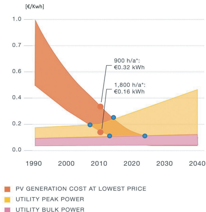
Figure 11.50 | Schematic representation of grid parity points (in blue, see text). *h/a: Hours of sun per annum, 900 h/a corresponds to northern countries of Europe. 1800 h/a corresponds to southern countries of Europe. Source: European Photovoltaic Industry Association/Greenpeace International, 2011.
