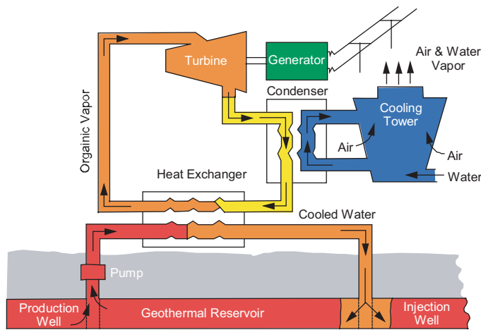
Figure 11.32 | Binary power or organic Rankine cycle plant using a low temperature geothermal resource and a secondary fluid of a low boiling-point hydrocarbon. Source: modified from Lund, 2007.
