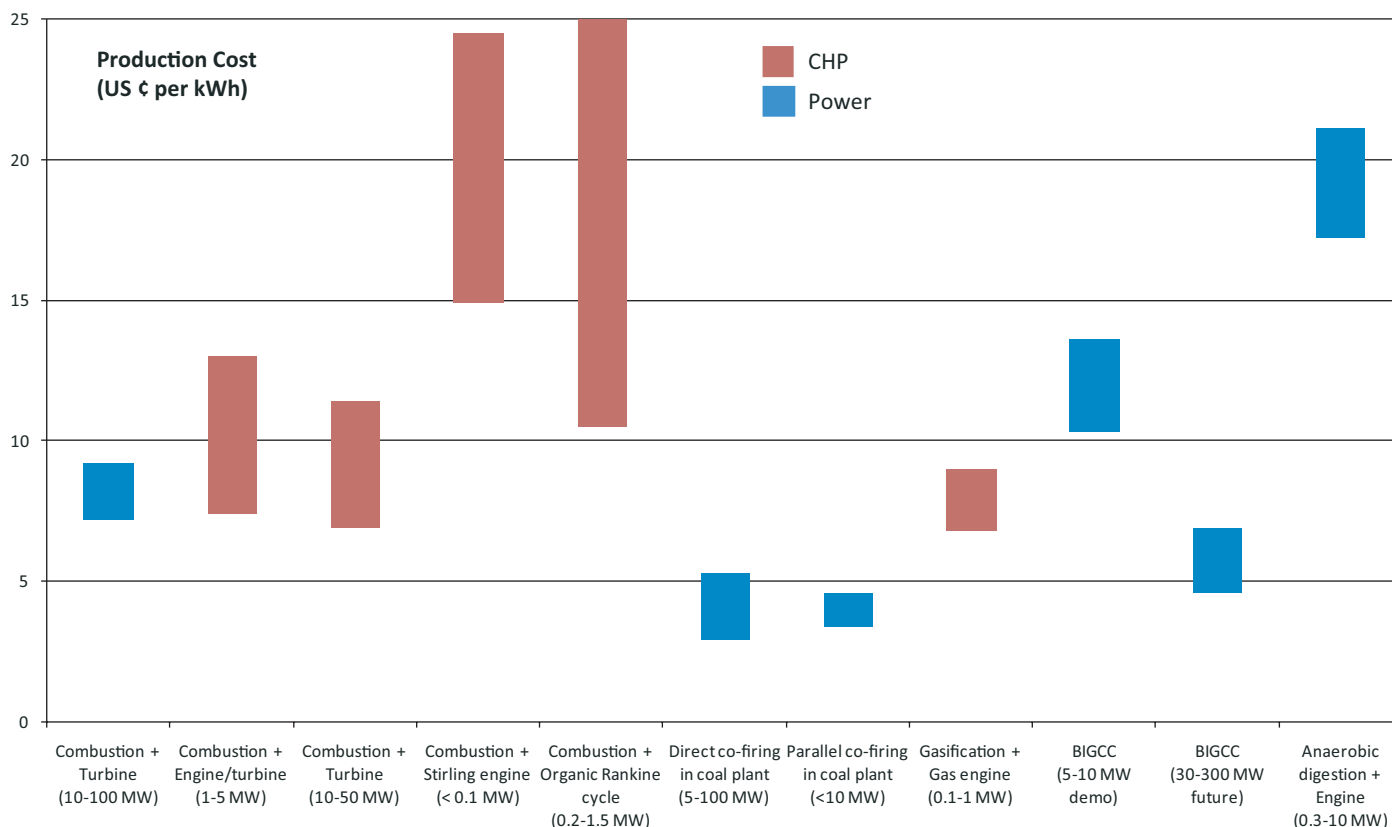
Figure 11.16 | Projected production costs for biomass to power and to CHP. Anaerobic digestion can also be operated in CHP mode; production cost will reduce by 60–80% (depending on technology and plant size) if “free” biomass feedstock is used, such as MSW, manure, or wastewater. Source: based on Bauen et al., 2009.
