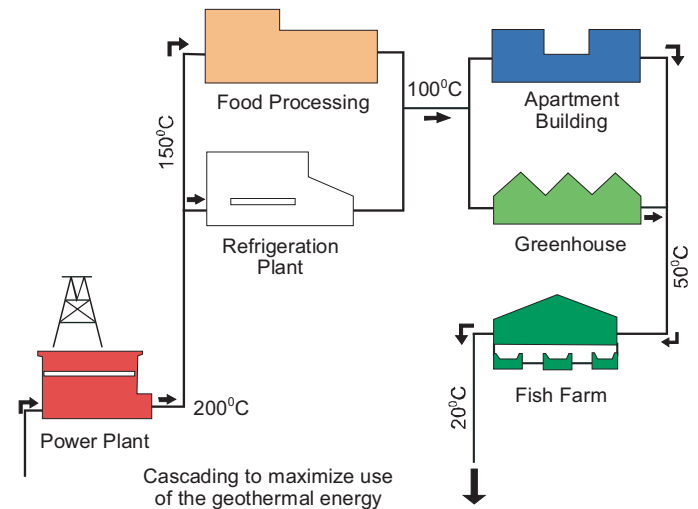
Figure 11.33 | Cascading the use of a geothermal resource for multiple applications. Source: Geo-Heat Center, 2003.
