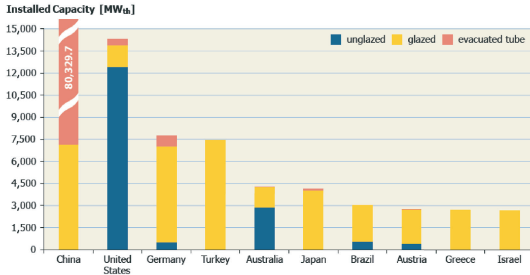
Figure 11.60 | Total capacity of solar collectors, 2008, in top 10 countries. Source: Weiss and Mauthner, 2010.
