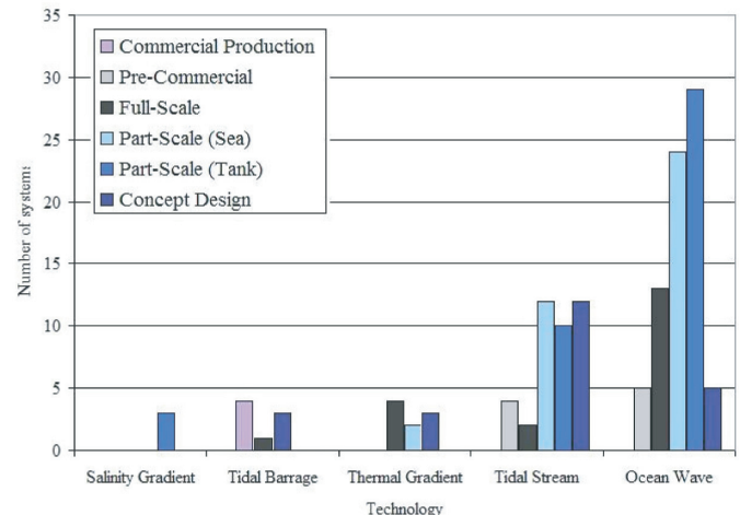
Figure 11.65 | Number of ocean energy conversion schemes and their maturity. Source: Kahn and Bhuyan, 2009.
