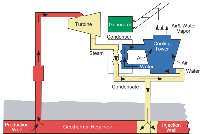
Figure 11.30 | Steam plant using a vapor or dry steam dominated geothermal resource. Source: modified from Lund, 2007.
