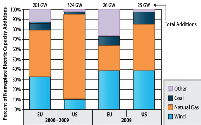
Figure 11.39 | Relative contribution of generation types to capacity additions in the United States and the European Union, 2000–2009 and 2009. Source: Wisner and Bolinger, 2010; EWEA, 2010.
