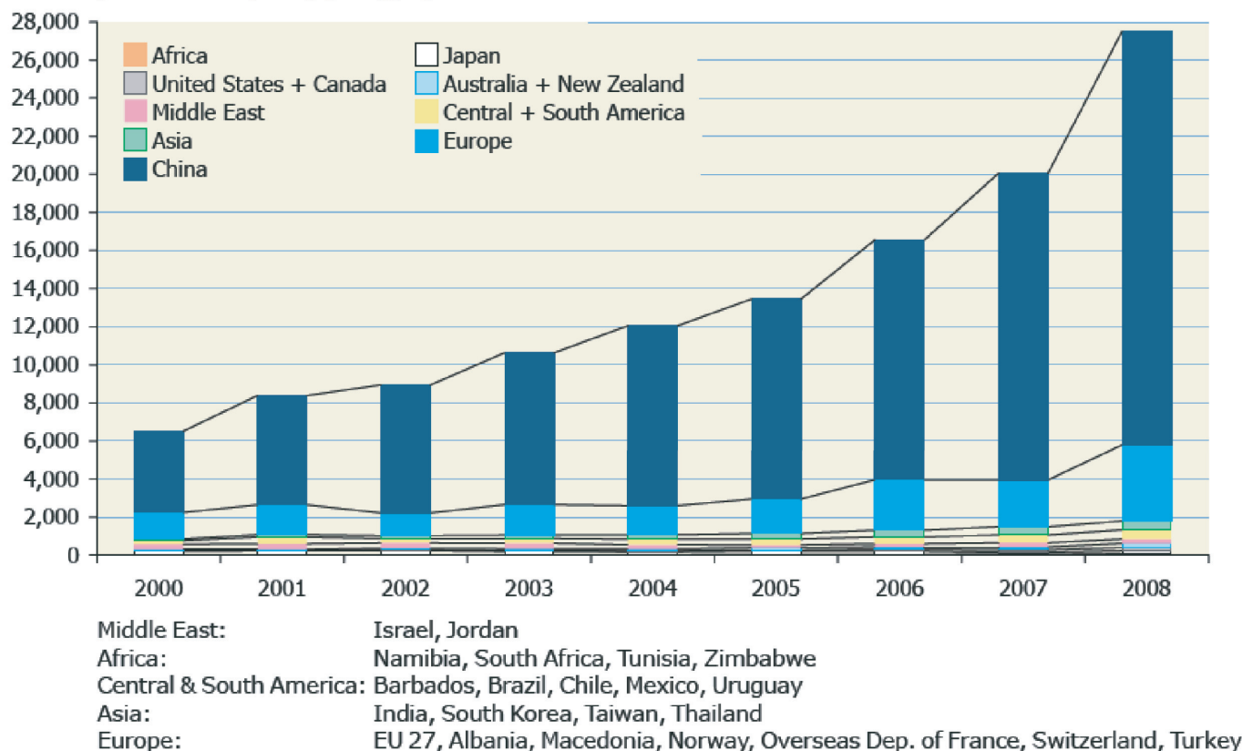
Figure 11.61 | Annual installed capacity of flat-plate and evacuated tube collectors, 2000–2008, total and per region. Source: Weiss and Mauthner, 2010.
