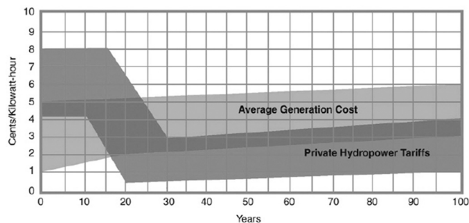
Figure 11.23 | Hydropower tariff versus average electricity generation costs in US 2008 ¢/kWh. Source: Trouille and Head, 2008.
