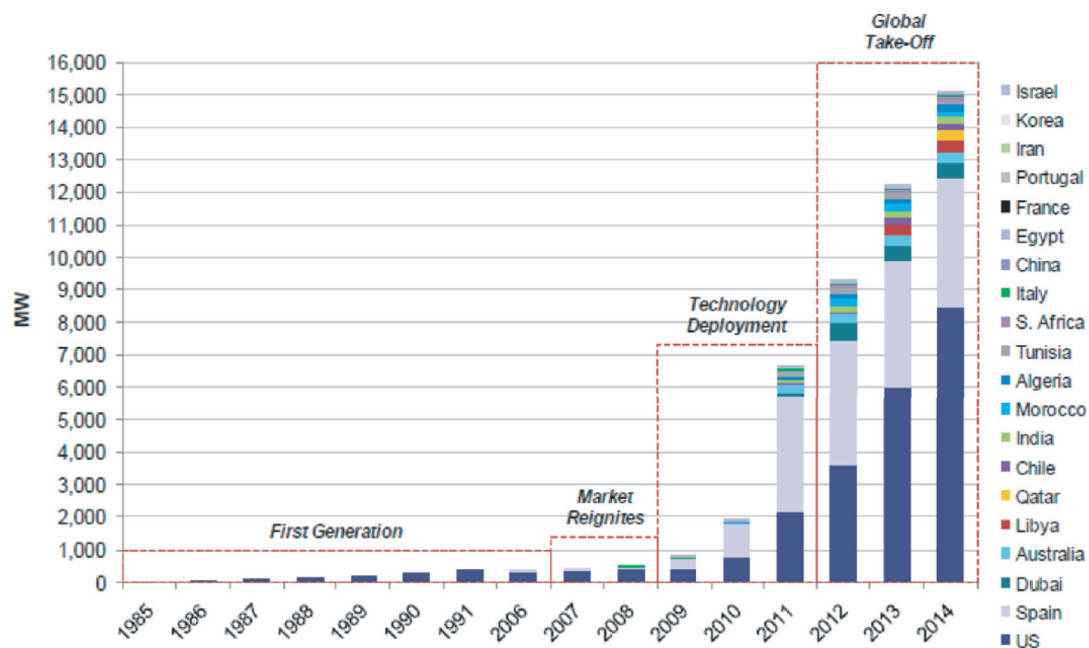
Figure 11.53 | CSP development, 1985–2008, project pipeline by country, 2009–2014. Source: IHS EER, 2009.
