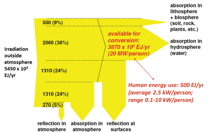
Figure 11.3 | The solar resource and its flows on Earth. The amount of solar energy available on Earth (estimated at 3.9 million EJ/yr) is many times the present human energy use (~528 EJ in 2009).
