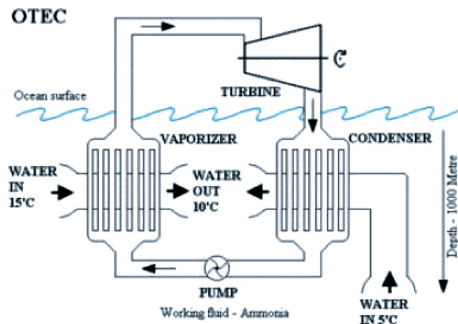
Figure 11.69 | A closed cycle OTEC power plant. Source: Sørensen and Weinstein, 2008.
