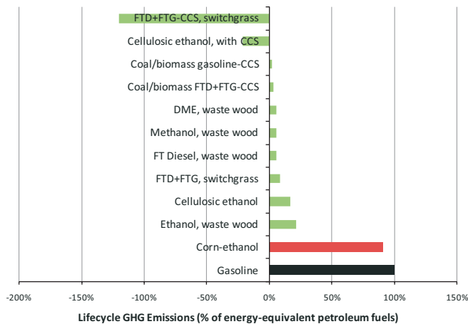
Figure 11.21 | Estimated life-cycle GHG emissions for second generation-biofuels, excluding any impacts of land use change. Estimates for fuels from waste wood are from CONCAWE et al. (2008). The corn-ethanol estimate represents the low estimate from Figure 11.20. The cellulosic ethanol estimates are based on Figure 12.22 in Chapter 12. The ethanol case with CCS assumes capture and storage of fermentation CO 2 . Others are based on Table 12.15 in Chapter 12. FTD + FTG refers to synthetic diesel and gasoline made via Fischer-Tropsch synthesis. DME is dimethyl ether.
