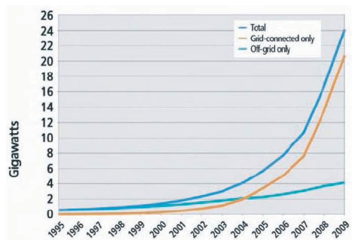
Figure 11.44 | Cumulative installed PV capacity, 1995–2009. In 2010 the total installed capacity was 40 GW (REN21, 2011). Source: REN21, 2010.
