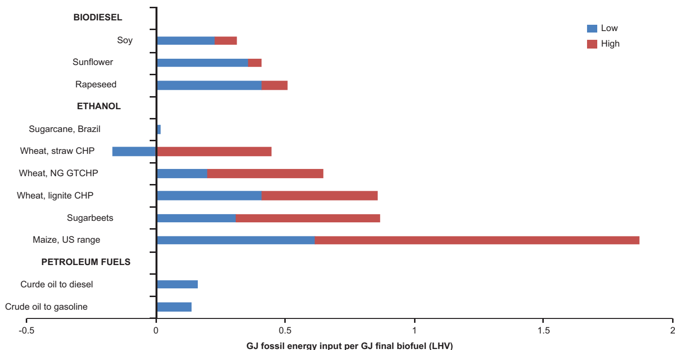
Figure 11.19 | Lifecycle fossil energy use estimates in production of several first generation biofuels and two petroleum fuels. Source: based on CONCAWE et al., 2008; Pradhan et al., 2009; Sheehan et al., 1998b; Farrell et al., 2006.
