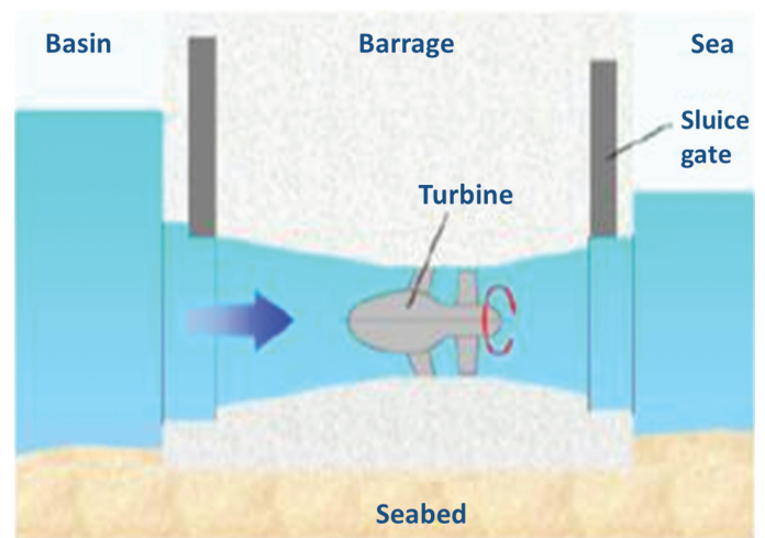
Figure 11.66 | Tidal barrage type of energy device. Source: Sørensen and Weinstein, 2008.
