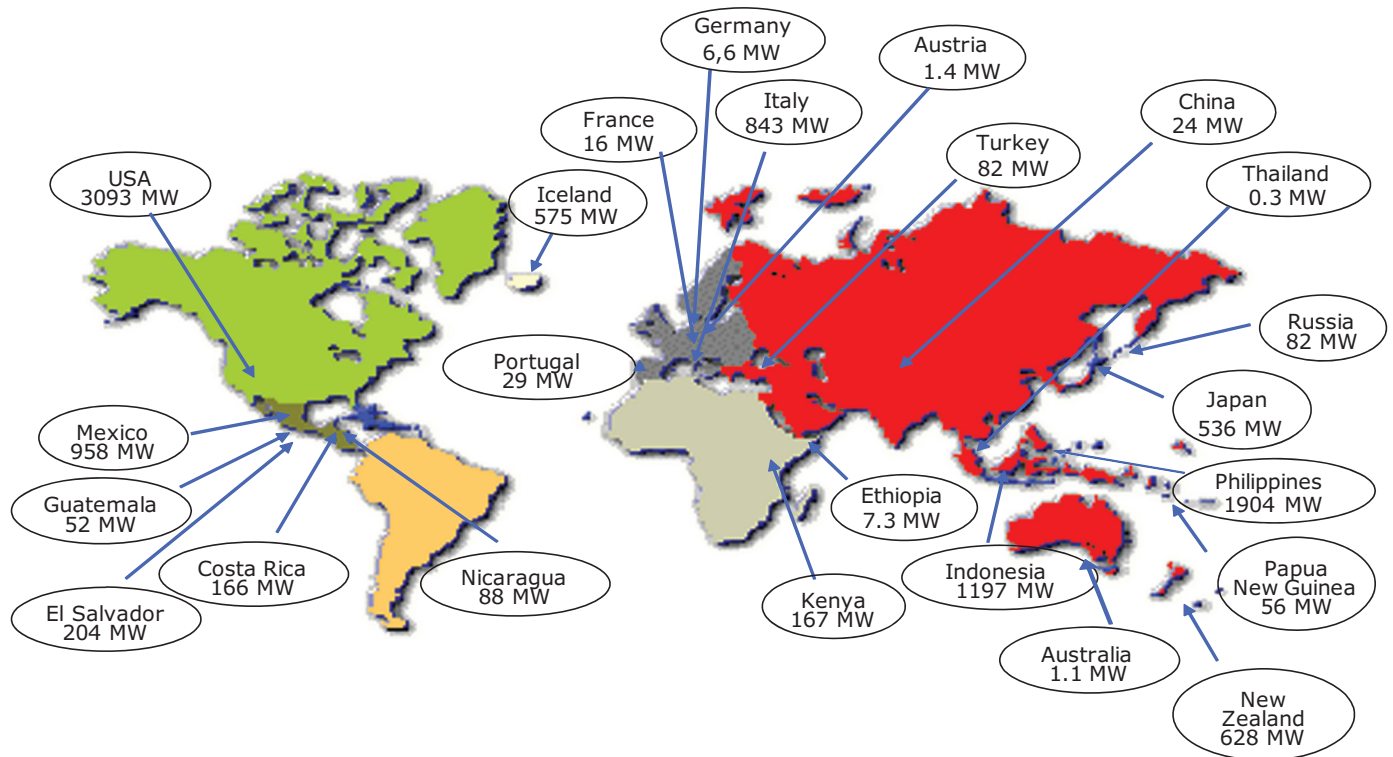
Figure 11.27 | Mapping of the 10.7 GW installed geothermal electric capacity in 2009. Source: data from Bertani, 2010.
