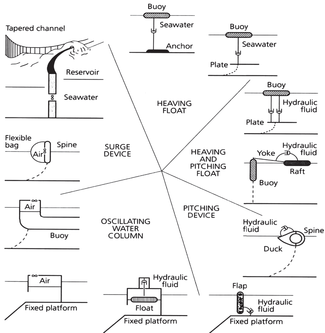
Figure 11.68 | Schematic representation of five mechanisms and 11 devices to use wave energy. Source: Cavanagh et al., 1993.
