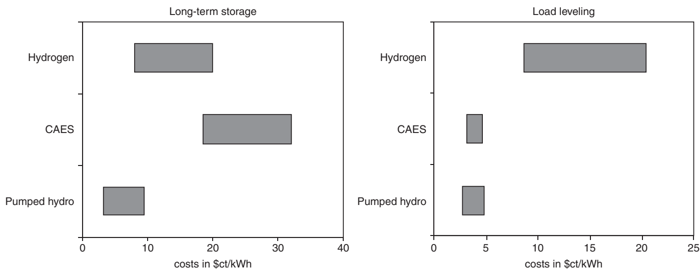
Figure 11.70 | Electricity storage costs for different storage options (US 2008 $/kWh). Source: Kleimaier et al., 2008; Leonard et al., 2008; Meiwes, 2009.
