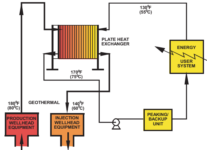
Figure 11.29 | Typical direct use geothermal heating system configuration. Source: based on Geo-Heat Center, 1998.
