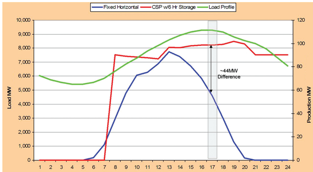
Figure 11.57 | Customer load profile (green) and power production profile of a CSP system with storage (red) and a non-tracking PV system (blue) over 24 hours. Source: Courtesy of Arizona Public Service.
