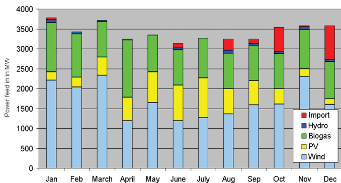
Figure 11.74 | Renewable energy mix of the Combi-Plant: simulation for 2006. Source: Mackensen et al., 2008.
