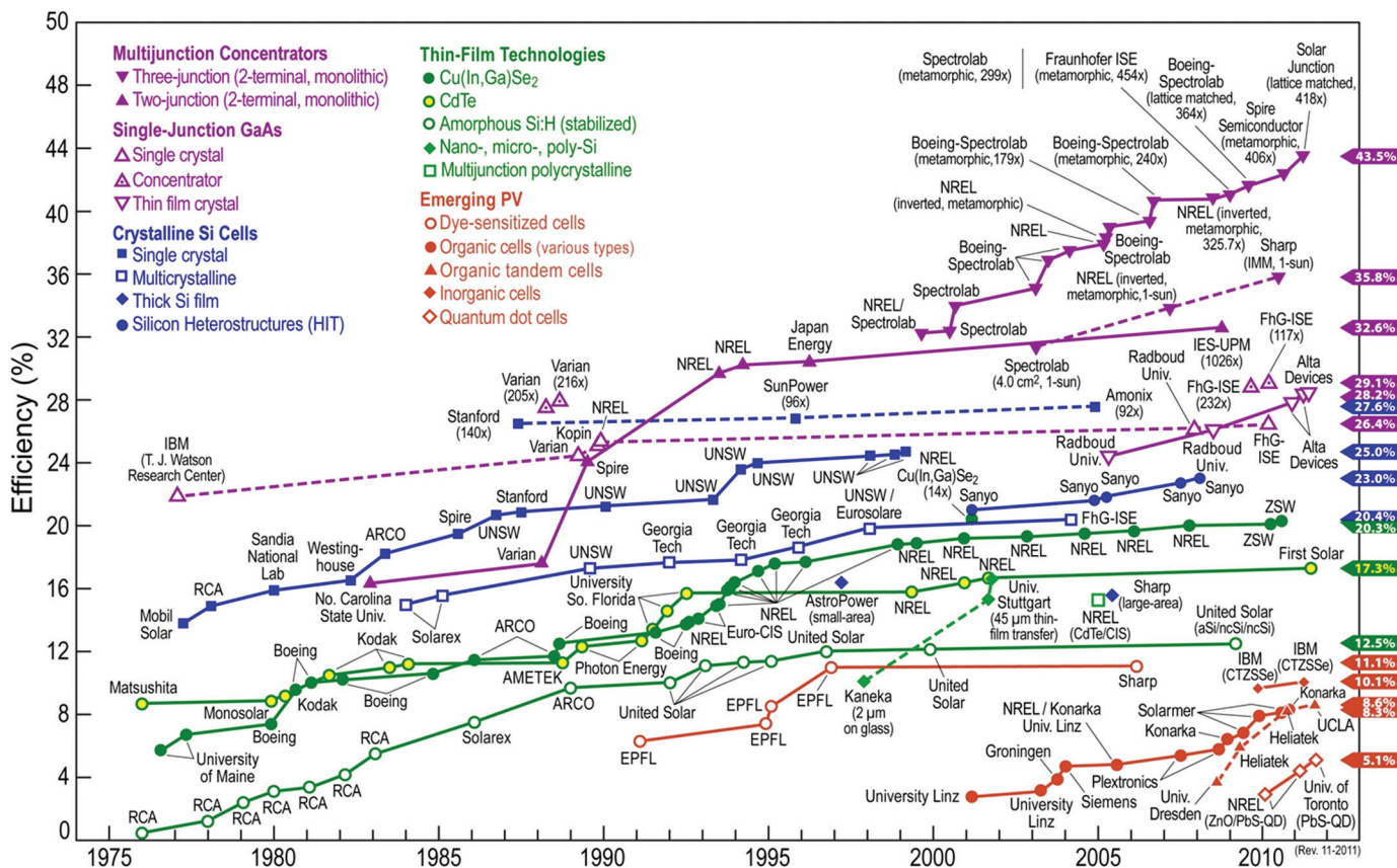
Figure 11.47 | Trends in conversion efficiencies for various laboratory solar cell technologies. Source: Kazmerski, 2011. Courtesy of NREL.
