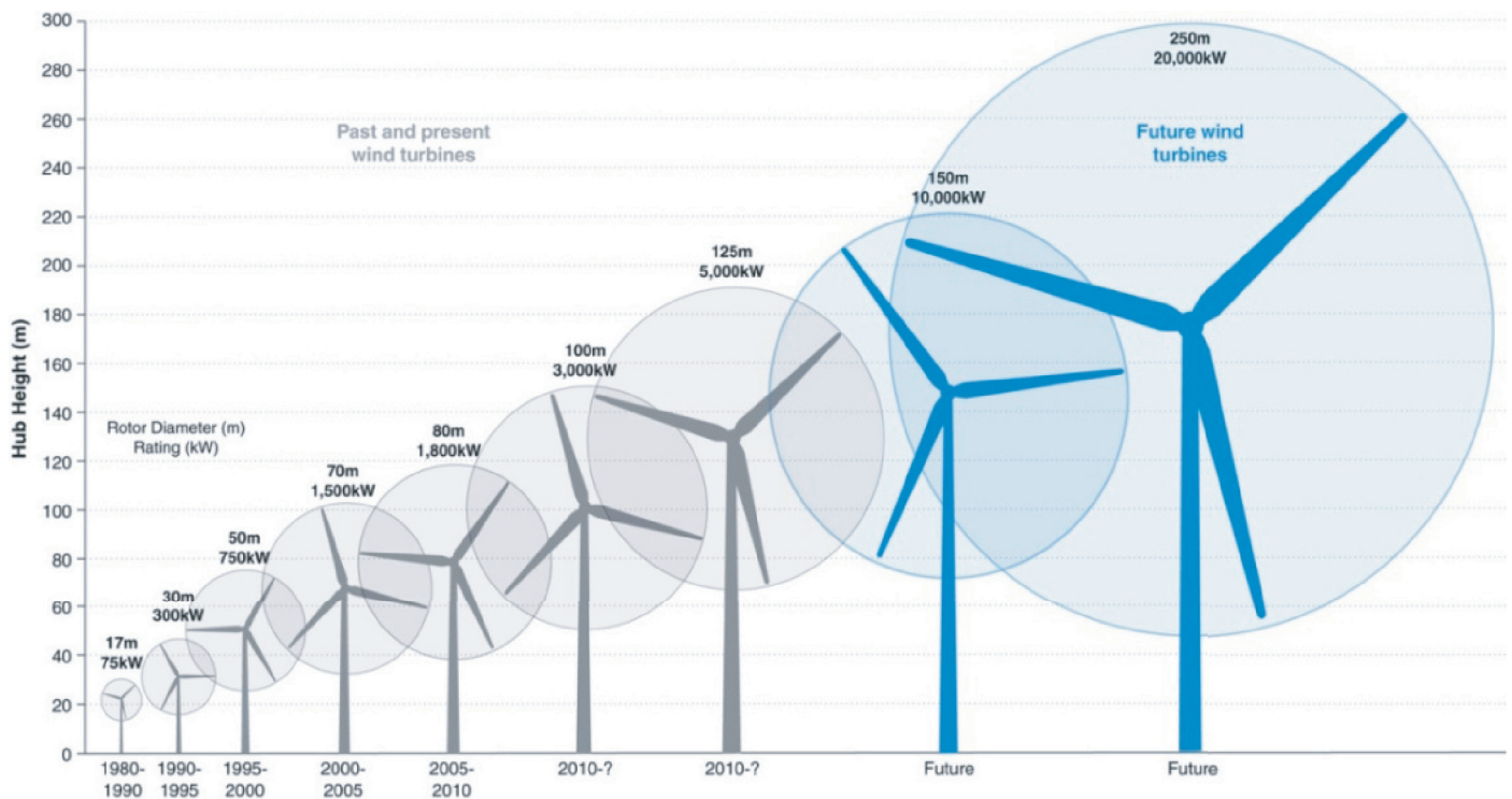
Figure 11.40 | Development and size growth (rotor diameter) of wind turbines since 1980. Source: courtesy of NREL.
