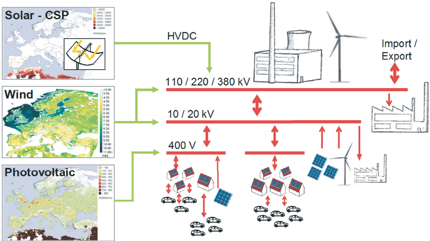
Figure 11.71 | Integration of renewables and electric vehicles into a supply system. Source: Sketch provided by Yvonne Scholz, German Aerospace Centre, 2011.
