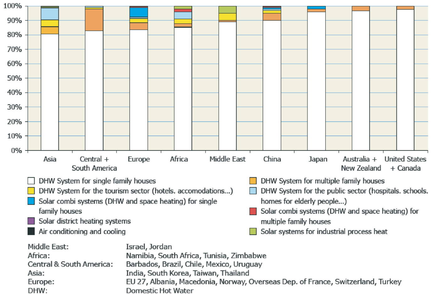
Figure 11.62 | Applications of glazed and evacuated tube collectors, by region, 2008. Source: Weiss and Mauthner, 2010.
