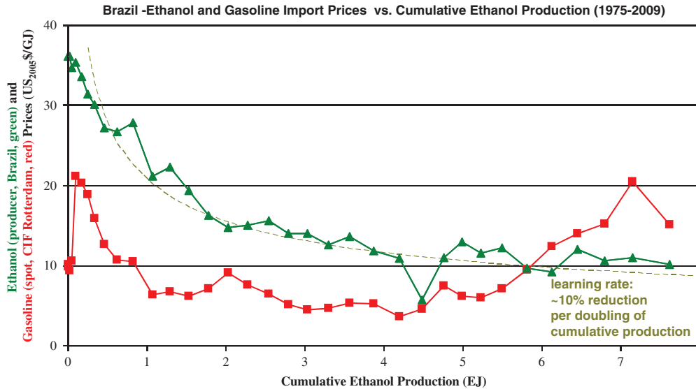
Figure 11.17 | Selling price for ethanol in Brazil versus cumulative production, compared with Rotterdam price for gasoline. Source: Mytelka and de Sousa Jr., 2011; see also van den Wall Bake et al., 2009.
