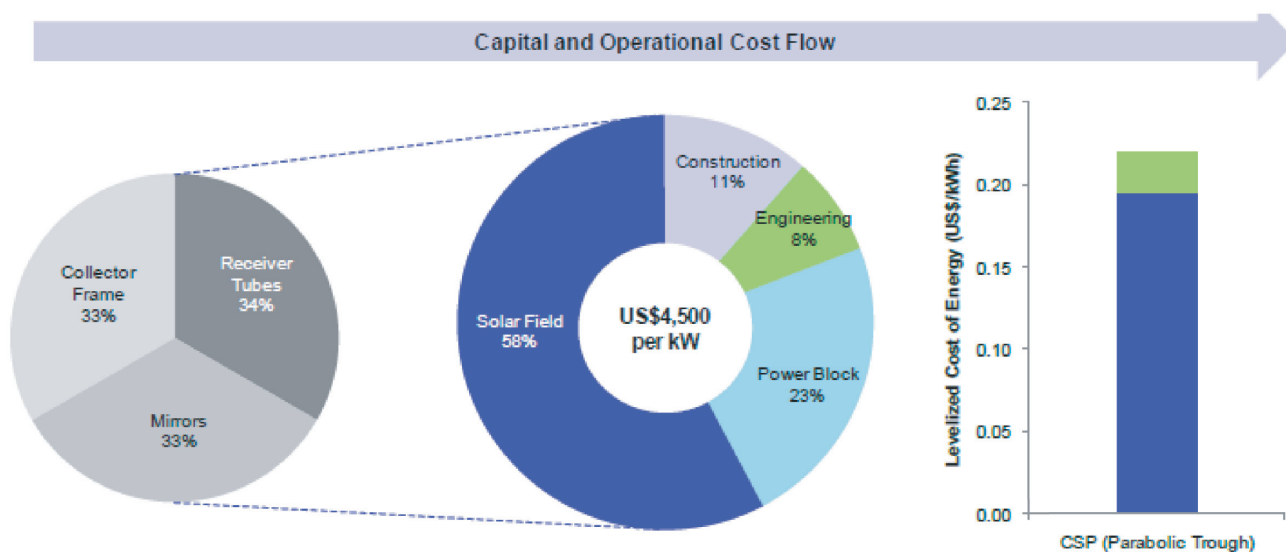
Figure 11.58 | Capital cost breakdown for parabolic trough plant. Source: IHS EER, 2009.
