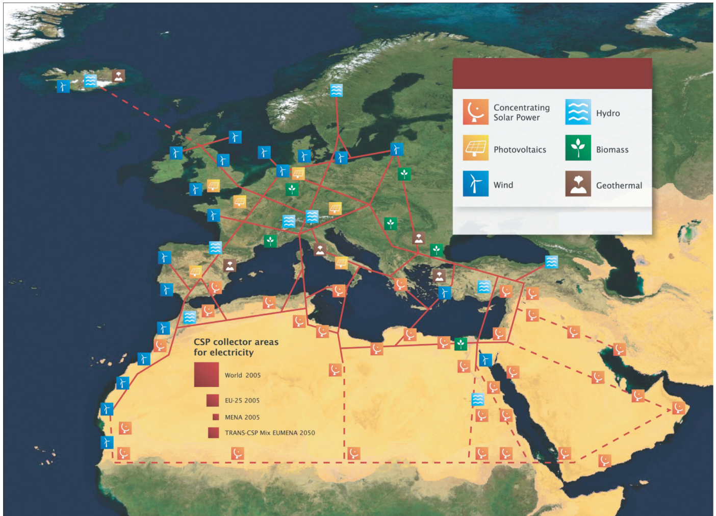
Figure 11.59 | Super grid envisioned by DESERTEC to bring power from the Middle East and North Africa to population centers throughout the region and in Europe. Source: DESERTEC Foundation, 2010.
