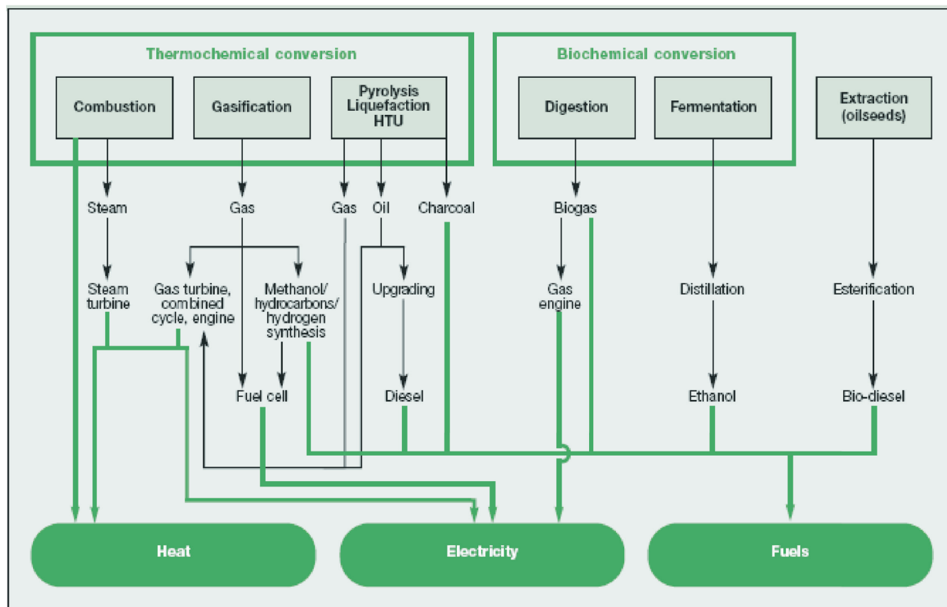
Figure 11.11 | Main conversion routes for biomass to secondary energy carriers. Source: UNDP et al., 2000.
