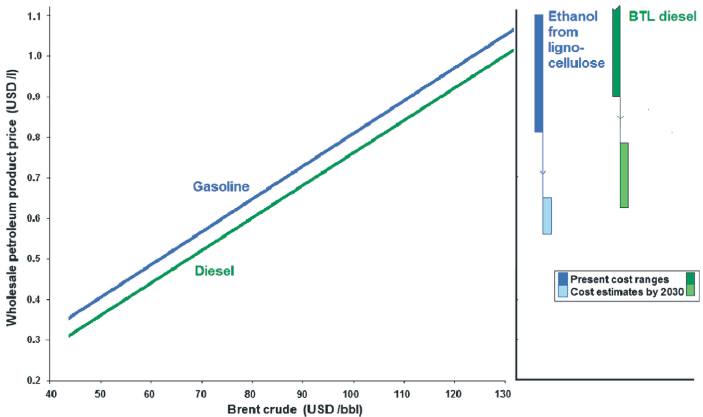
Figure 11.18 | Range of production cost estimates for second-generation biofuels (in US 2006 $ per liter of gasoline equivalent). The 2030 estimates assume significant investment in RD&D. Source: Sims et al., 2010.
