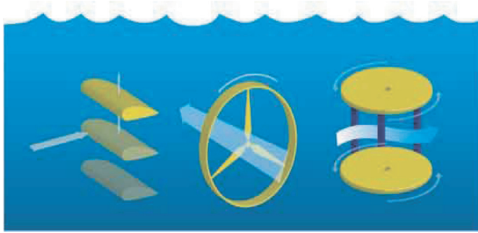
Figure 11.67 | Three technologies to convert ocean current energy: reciprocating hydrofoil (left), horizontal axis turbine (middle), vertical axis turbine (right). Source: DP Energy, 2010.
