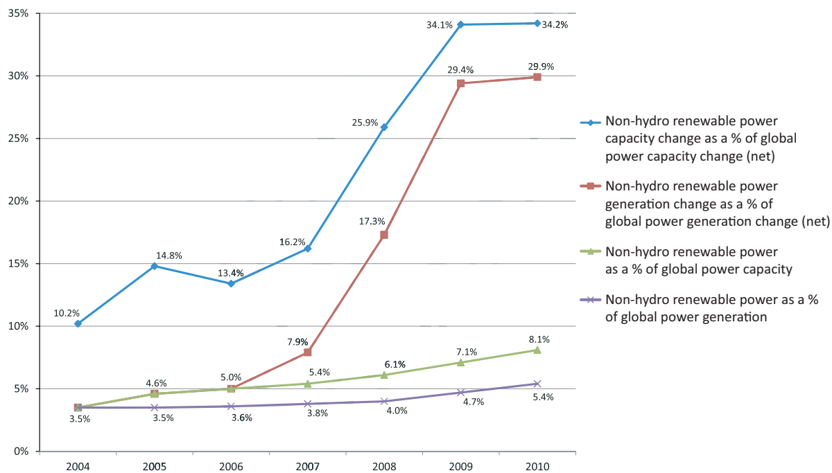
Figure 11.1 | The generating power and capacity of non-hydropower renewable energy sources as a proportion of global power generation and capacity in the period 2004–2010. Source: UNEP and BNEF, 2011.
