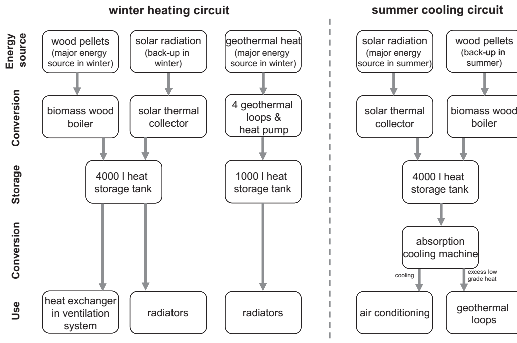
Figure 11.76 | Renewable heating and cooling system in the Renewable Energy House, Brussels, Belgium. Source: adopted from EREC, 2008.
