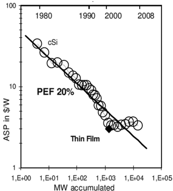
Figure 11.49 | PV module experience curves showing the average selling price (ASP) of modules in US 2008 $ as a function of the cumulative module production. Note that the Progress Ratio (or PEF: Price Experience Factor) is about 20%. See text for further explanation of the curve. Source: Hoffmann et al., 2009.
