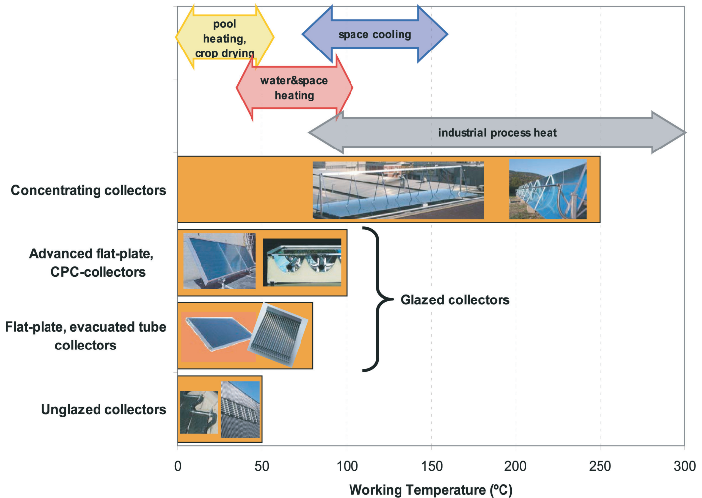
Figure 11.63 | Active solar thermal technologies, collectors, and working temperature ranges. Source: IEA-CERT, 2011. Courtesy of ORNL.
