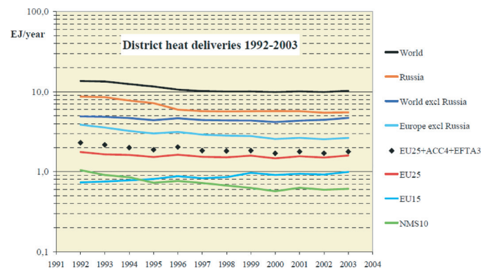
Figure 11.75 | Development of district heat in various parts of the world, 1992–2003. Source: Ecoheatcool, 2005–2006.
