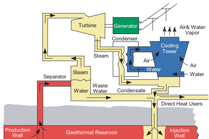
Figure 11.31 | Single-stage flash steam plant using a water-dominated geothermal resource with a separator to produce steam. Source: modified from Lund, 2007.
