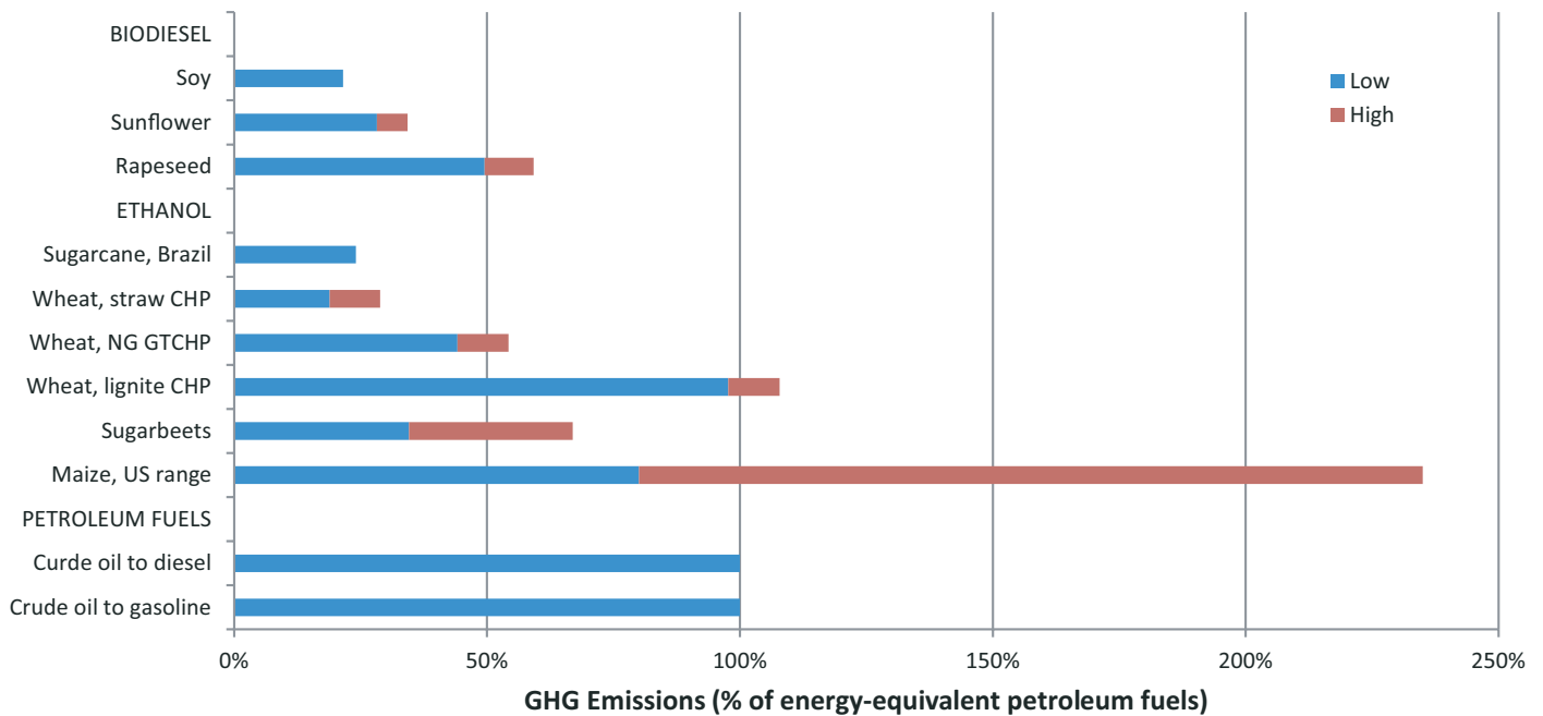
Figure 11.20 | Estimated life-cycle GHG emissions for first-generation biofuels, excluding any impacts of land use change. Source: based on CONCAWE et al., 2008; Pradhan et al., 2009; Sheehan et al., 1998b; Farrell et al., 2006; Macedo et al., 2008. The low and high values for maize ethanol are based on analysis by Shapouri et al. (2002) and Pimental and Patzek (2005), respectively, as reported by Farrell et al. (2006).
