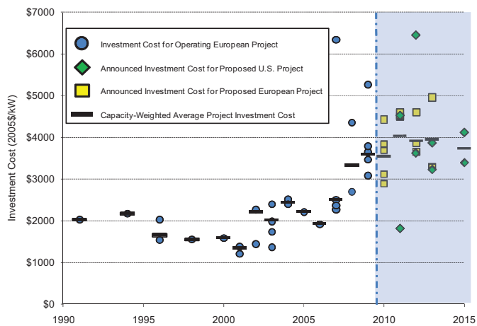
Figure 11.42 | Capital costs for installed and announced offshore wind projects. Source: Musial and Ram, 2010. Courtesy of NREL.
