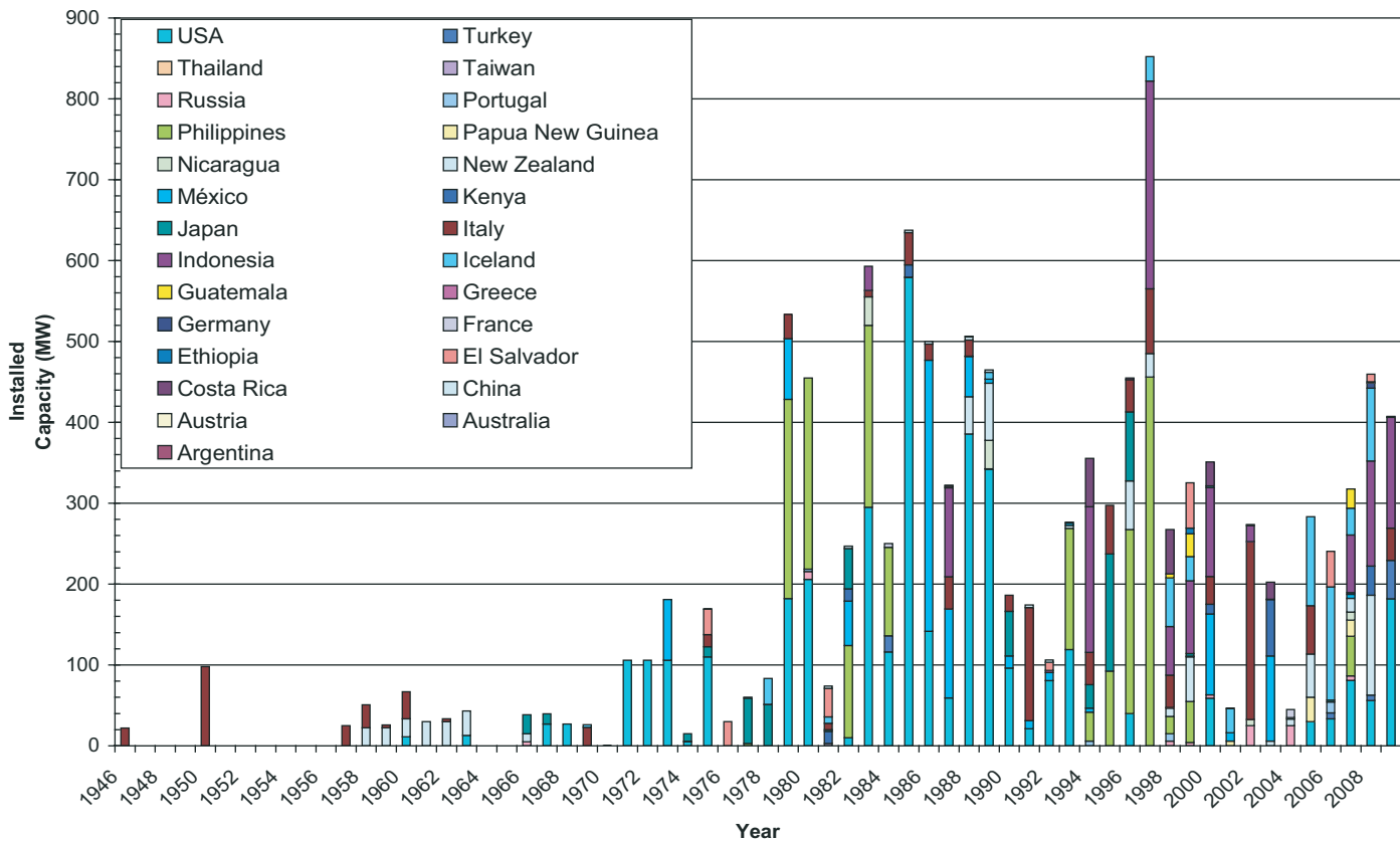
Figure 11.25 | Installed geothermal electricity capacity, 1946–2010, by country and in total. Source: data from Bertani, 2010.
