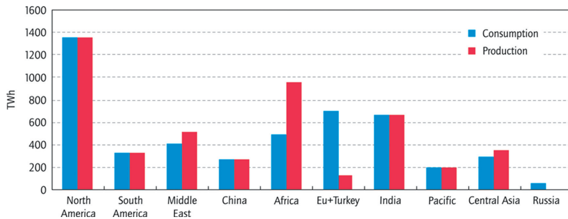
Figure 11.52 | Possible production and consumption of CSP electricity in 2050. Source: IEA, 2010e. ©OECD/International Energy Agency 2010.
