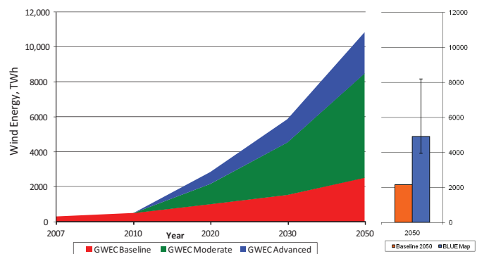
Figure 11.36 | Wind energy generation estimates from two studies (left panel: GWEC and Greenpeace, 2010a; right panel: IEA, 2010a).
