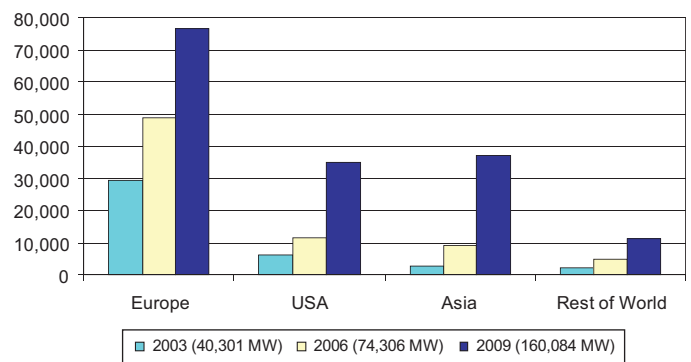
Figure 11.37 | Cumulative installed capacity in Europe, United States, Asia, and the rest of the world, 2009. Source: BTM Consult, 2010; AWEA project database for US capacity.
