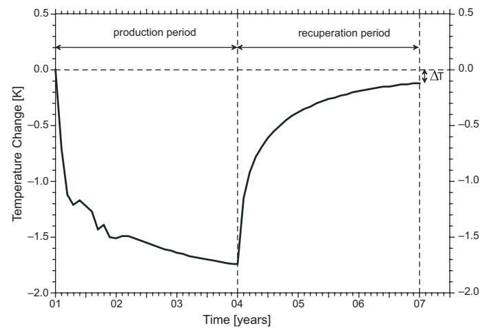
Figure 11.34 | Calculated ground temperature change at a depth of 50 m and at a distance of 1 m from a 105 m long borehole heat exchanger over a production period and a recuperation period of 30 years each. Source: Eugster and Rybach, 2000.
