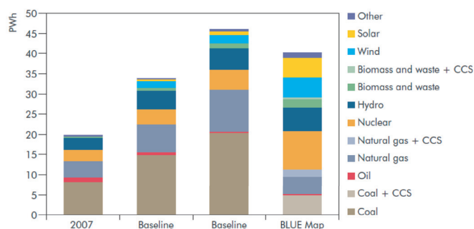
Figure 11.5 | The contribution of different energy sources to the global electricity supply in the Baseline and the BLUE Map scenario developed by IEA. Source: IEA, 2010a. ©OECD/International Energy Agency 2010.
