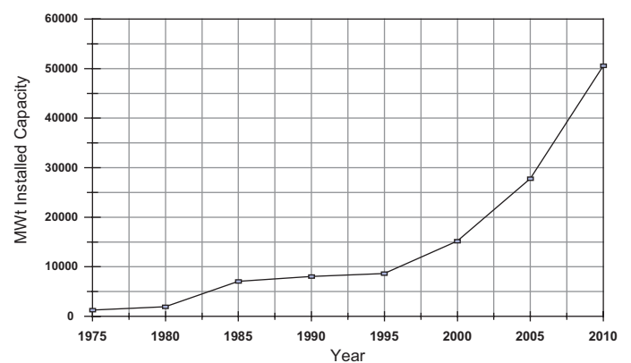
Figure 11.28 | Worldwide growth of installed capacity of geothermal direct use. Source: Lund et al., 2010.
