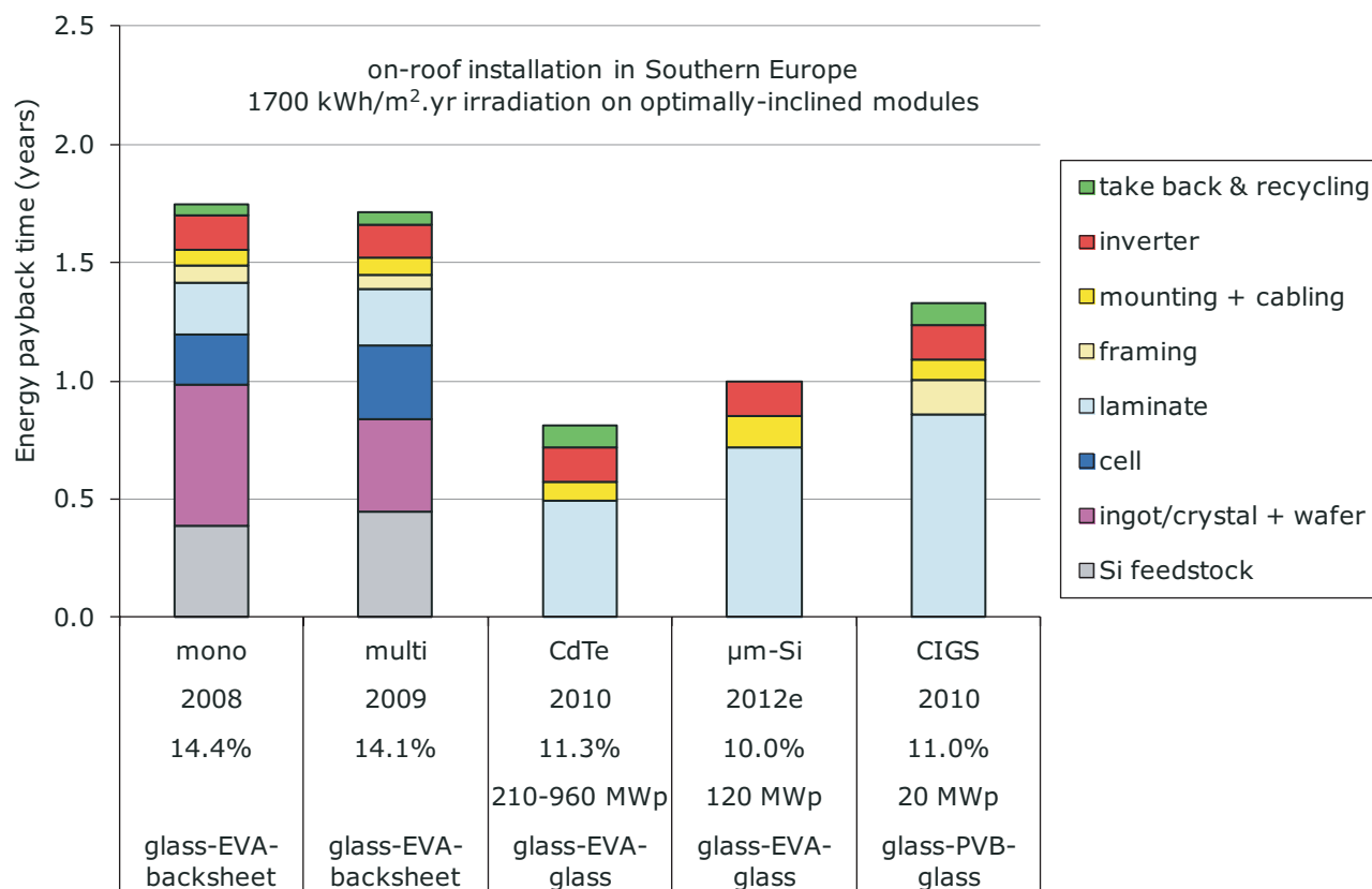
Figure 11.51 | Energy payback time (EPBT) of on-roof PV systems for an in-plane irradiation of 1700 kWh/m 2 /yr. Source: de Wild-Scholten, 2011.
