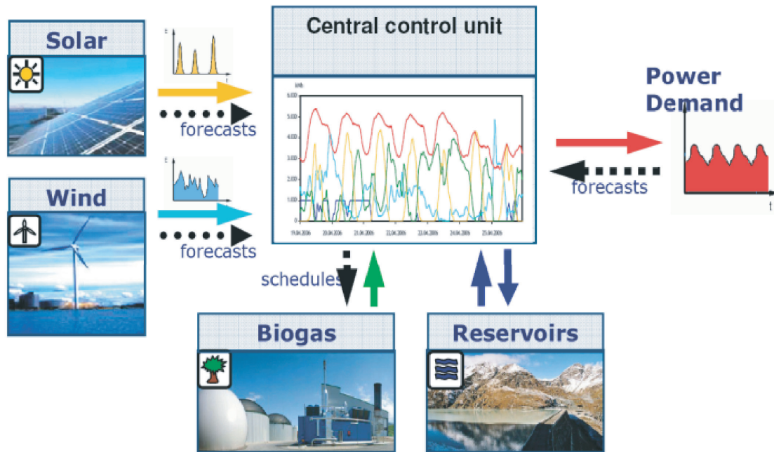
Figure 11.73 | The Renewable Combi-Plant. Source: Mackensen et al., 2008.
