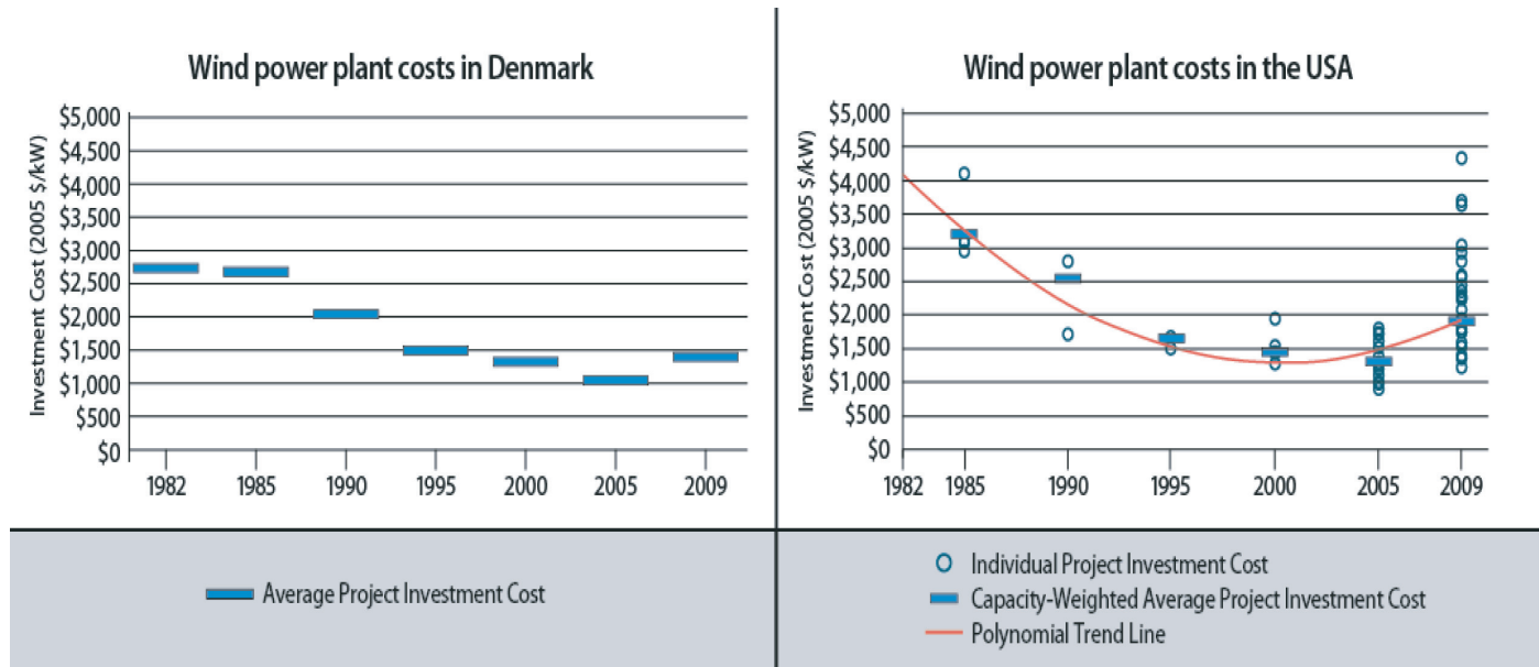
Figure 11.41a, b | Installed Wind Project Costs over time in Denmark and the United States. Source: Denmark: Nielson et al., 2010; United States: Wisner and Bolinger, 2010.
