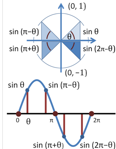
(Top): Trigonometric function \sin \theta for selected angles \theta , \pi - \theta , \pi + \theta , and 2\pi - \theta in the four quadrants. (Bottom) Graph of sine function versus angle. Angles from the top panel are identified.
