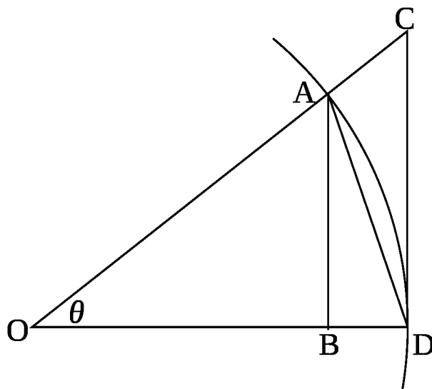
Illustration of the sine and tangent inequalities.
