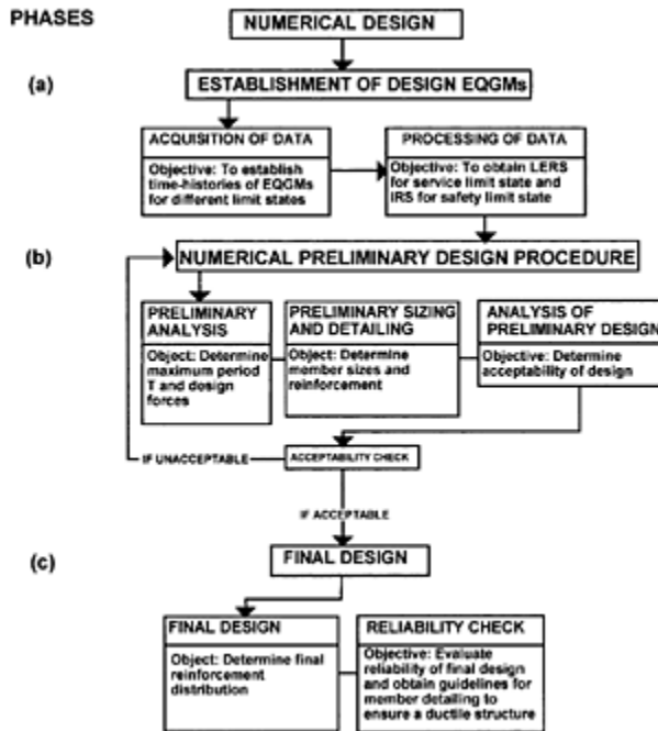
FIGURE 8.1 Steps of the numerical design.
