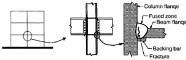
FIGURE 15.1 Common zone of fracture initiation in a typical beam-column connection.
