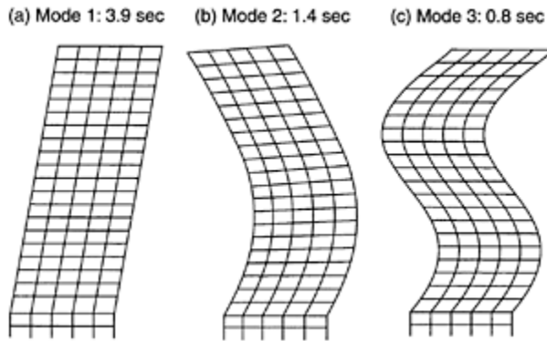
FIGURE 6.28 Lower three vibration modes and periods of 20-story building.
