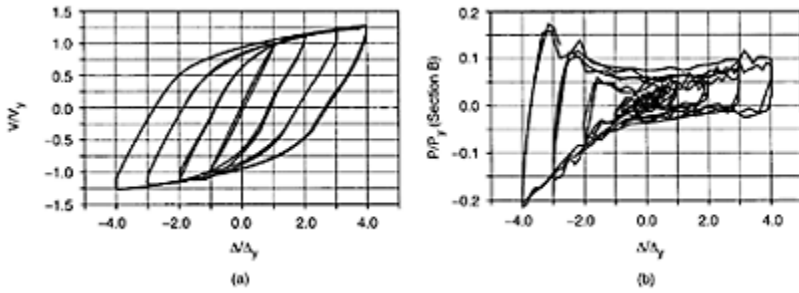
FIGURE 16.39 Measured hysteresis response, (a) Global response; (b) round hollow structural section casing response. (Tremblay, R., Degrangé, G. and Blouin, J. (1999). Seismic rehabilitation of a four-story building with a stiffened bracing system, Proc. 8th Canadian Conference on Earthquake Engineering , Vancouver, BC, 549–554.)
