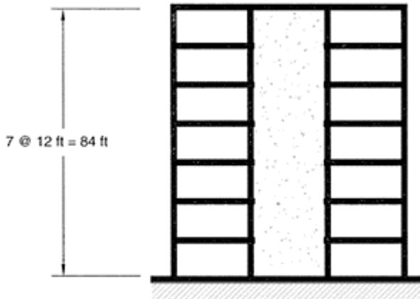
FIGURE 13.3 Frame with dominant wall.
