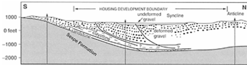
FIGURE 3.7 Diagrammatic cross section through Moorpark housing development. Sespe Formation: bedded sedimentary rocks largely of middle Tertiary age. Overlying strata are Quaternary in age, consisting of a basal marine sandstone, overlying marine claystone, and non-marine gravels. Deformed gravels are probably no younger than 500,000 years. Heavy lines show low-angle thrusts on south limb of syncline. These thrusts were interpreted as shallow, emerging from the claystone layer, rather than continuing downward to seismogenic depths and comprising independent earthquake sources. “Undeformed gravels” are cut by faults and are locally tilted, but displacement on faults nowhere exceeds 6 inches. Deep control provided by oil wells (derrick symbols and vertical lines); shallow control from trenches and borings.
