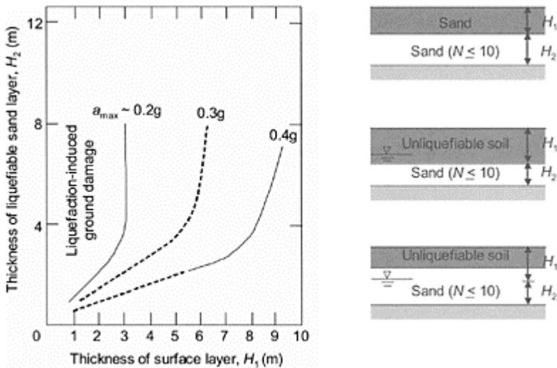
FIGURE 4.33 Empirical relationships for estimating conditions under which surficial evidence of liquefaction can be expected. Surficial evidence can be expected for H_1 – H_2 pairs that plot above each of the indicated curves. (From Ishihara, K., Proceedings, Eleventh International Conference on Soil Mechanics and Foundation Engineering , 1, 321–376, 1985. With permission.)
