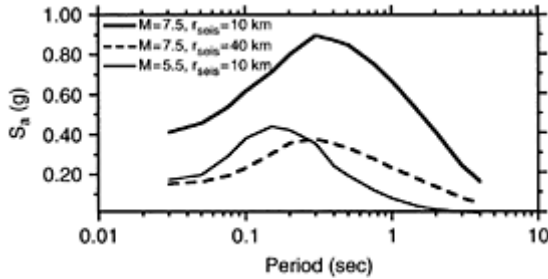
FIGURE 5.11 Pseudo-acceleration ( S_a ) spectra for the average of the two horizontal components for 5% damping at a stiff soil site and for strike-slip faulting, based on the Campbell and Bozorgnia (2003) ground motion (attenuation) relations. Here r_{seis} is the shortest distance from the site to the seismogenic rupture zone of the fault (see Section 5.4).
