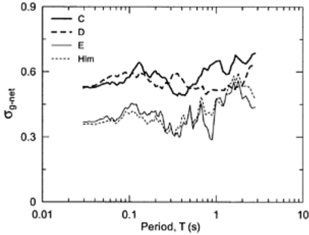
FIGURE 4.14 Variation with period of dispersion in ground response predictions associated with factors other than the ground response model estimation error for NEHRP Categories C-E and Holocene lacustrine/marine sediments (Him). (From Baturay, M.B. and Stewart, J.P. Bull Seism. Soc. Am. , 93, 2025–2042, 2003. With permission.)
