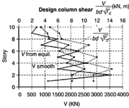
FIGURE 8.35 Shear and normalized shear stress for interior columns.
