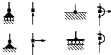
FIGURE 6.2 Typical support symbols for the 2d case.
