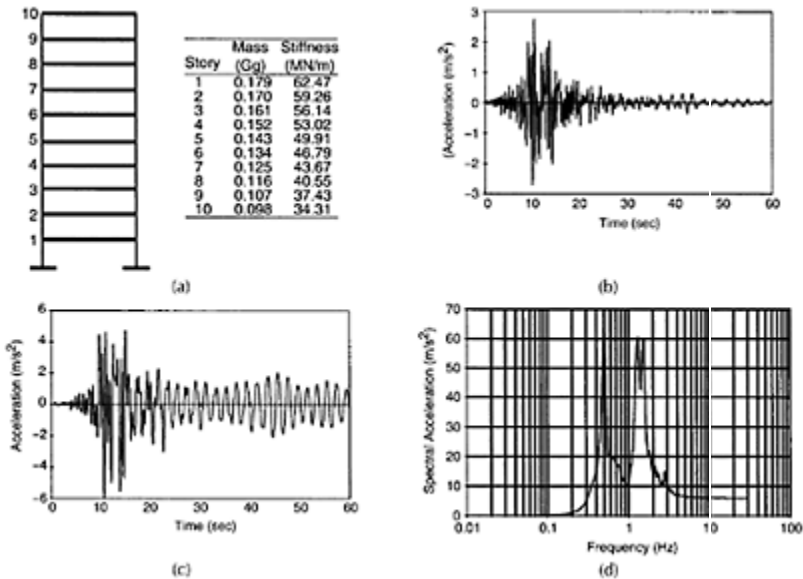
FIGURE 19.9 (a) Ten-story building considered in Example 19.1. (Note: Gg=68, 525 slugs; 1 \text{ MN/m}=737.5 \text{ kips/ft} ); (b) E-W component of ground acceleration recorded at the Foster City station during the 1989
