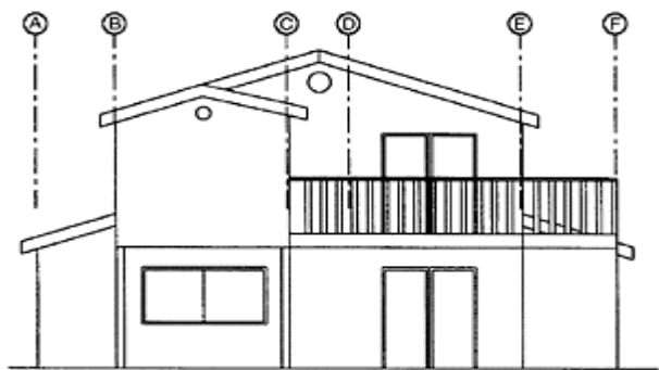
FIGURE 18.23 Large House Index Building, South Elevation. (From Isoda et al, 2002, CUREE Publication W-12, CUREE, Richmond, CA. With permission.)
