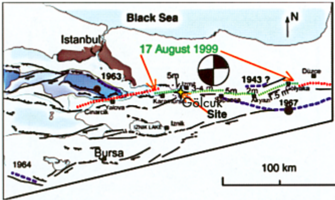
COLOR FIGURE 3.10 Map of the Istanbul, Turkey, region showing the 1999 surface rupture on the North Anatolian fault near the automobile assembly plant. Dashed lines in the Marmara Sea locate undersea faults that did not rupture in 1999 but have ruptured in previous cycles, including a large earthquake in 1766. An earthquake in 1894 may have ruptured an offshore fault at the eastern end of the Marmara Sea between Istanbul and the North Anatolian fault.
