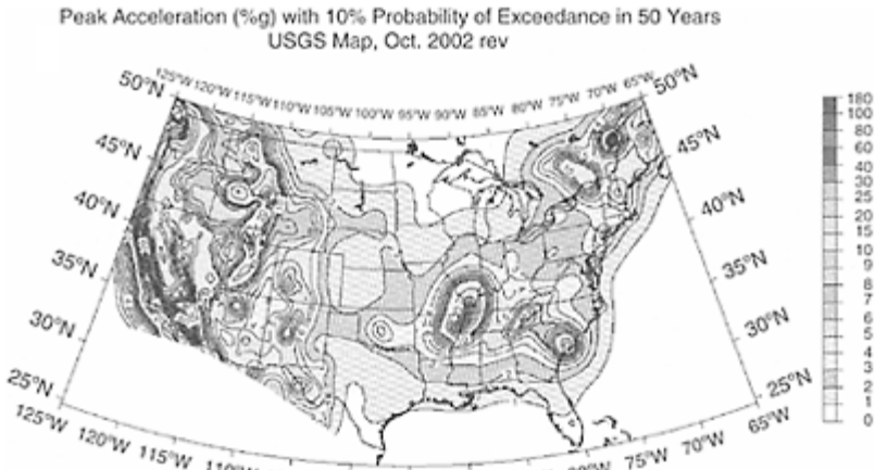
FIGURE 2.3 Recent seismic hazard map of the United States (after Frankel et al, 2002).
