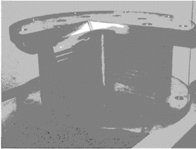
FIGURE 11.8 Cut-away model of a lead-plug isolation bearing (courtesy of DIS, Inc.).
