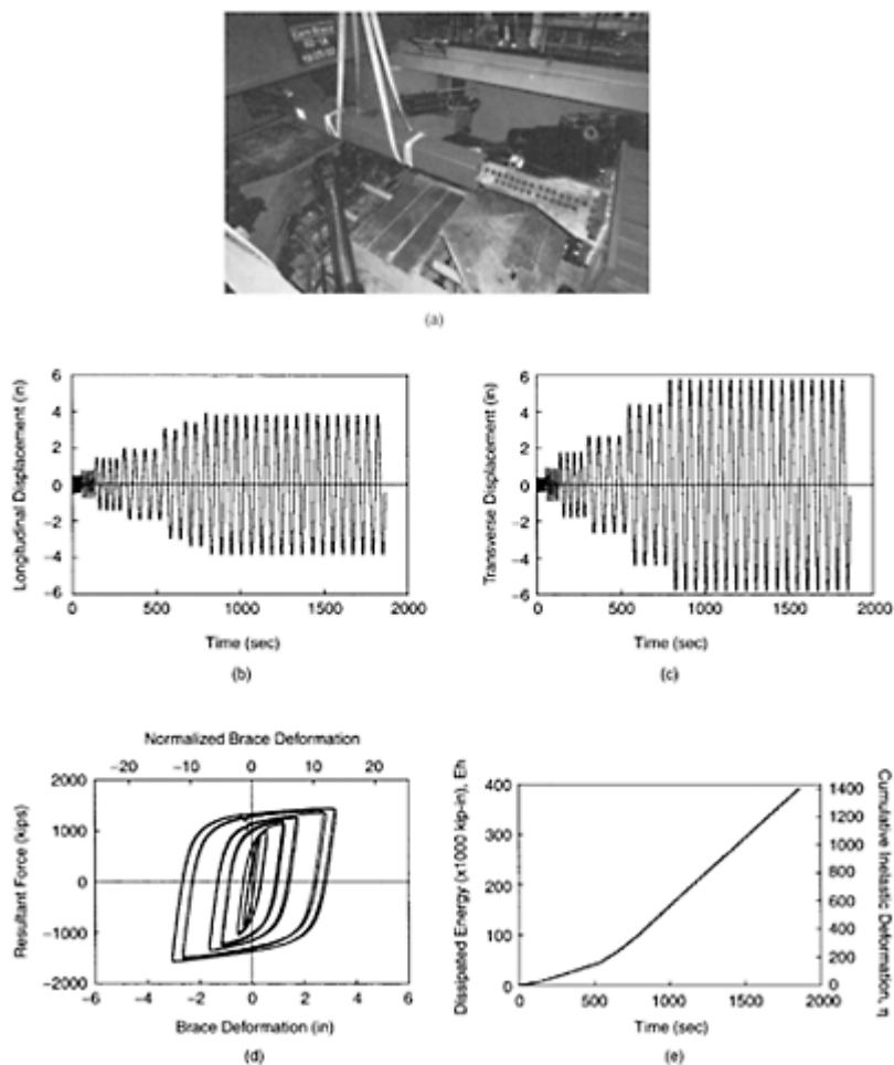
FIGURE 16.46 Subassembly testing of CoreBrace buckling- restrained braces, (a) Test setup; (b) longitudinal deformation; (c) transverse deformation; (d) hysteresis response; (e) dissipated energy and cumulative inelastic axial deformation capacity. (Merritt, S., Uang, C.M.
