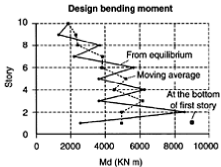
FIGURE 8.32 Design bending moment for interior column.
