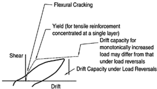
FIGURE 13.20 Drift capacity.
