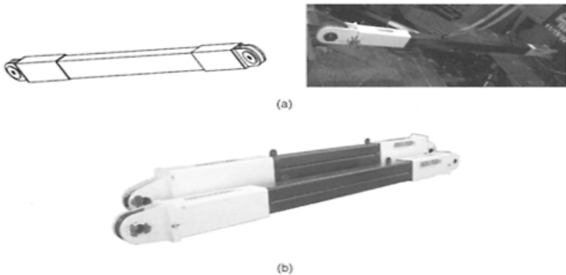
FIGURE 16.28 Star Seismic buckling- restrained brace . (a) Single-tube configuration; (b) multitube
