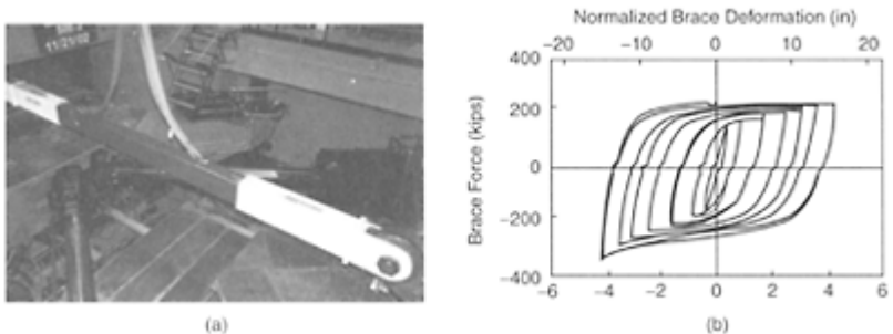
FIGURE 16.47 Test setup and typical response of Star Seismic buckling-restrained braces, (a) Test setup; (b) hysteresis response. (Merritt, S., Uang, C.M. and Benzoni, G. (2003b), Subassembly testing of Star Seismic buckling-restrained braces, Report
