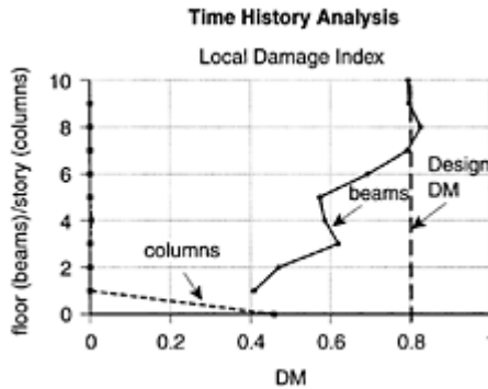
FIGURE 8.62 Maximum damage index at each level from time-history analysis.
