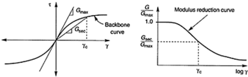
FIGURE 4.4 Relationship between (a) backbone curve and (b) modulus reduction curve.
