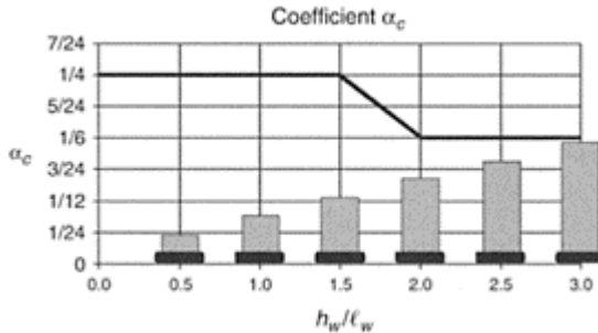
FIGURE 14.37 Coefficient \alpha_c for wall shear design.
