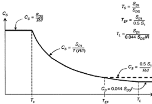
FIGURE 14.10 Seismic response coefficient, C_s , in the equivalent lateral force procedure.
