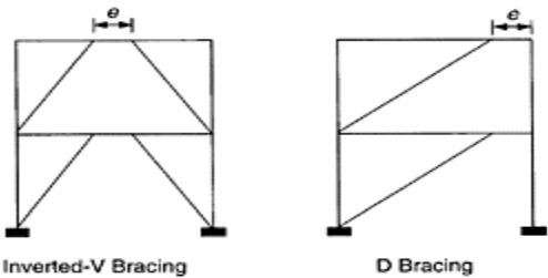
FIGURE 16.4 Examples of eccentric bracing configurations.
