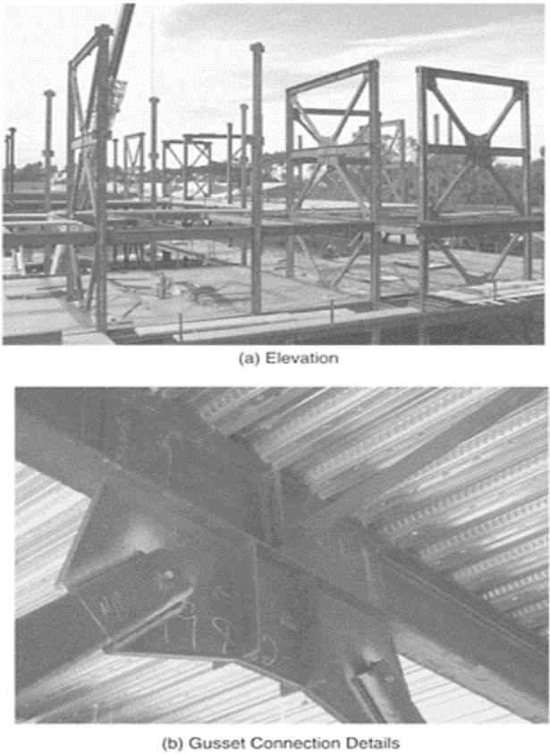
FIGURE 16.3 Special concentrically braced frame construction with X configuration.
