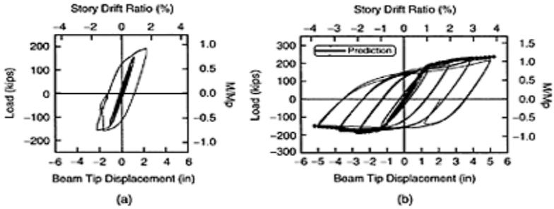
FIGURE 15.14 Load versus beam tip deflection relationships of the composite specimens (Yu, Q.-S., Noel, S. and Uang, C.-M. (1997). Experimental studies on seismic rehabilitation of pre-Northridge steel moment connections: RBS and haunch approach, Report No. SSRP-97/08, University of California, San Diego, CA).
