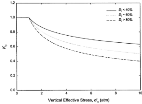
FIGURE 4.30 Variation of overburden correction factor, K_\sigma , with overburden pressure. (From Harder, L.F. and Boulanger, R.W., Proceedings, NCEER Workshop on Evaluation of Liquefaction Resistance of Soils , 167–190, 1997. With permission.)
