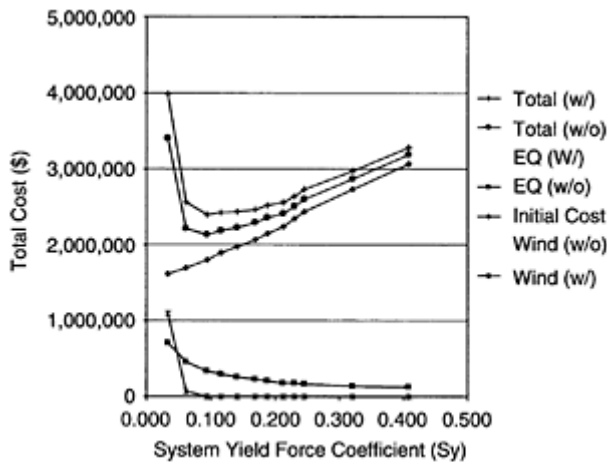
FIGURE 7.9 Life-cycle costs of a nine-story office building as function of system yield force coefficient at Seattle (life=50 year, discount rate=5%, w/ and w/o indicate with and without consideration of costs due to deaths and injuries). (Kang and Wen, Structural Research Series No. 629, University of Illinois at Urbana-Champaign, 2000.)
