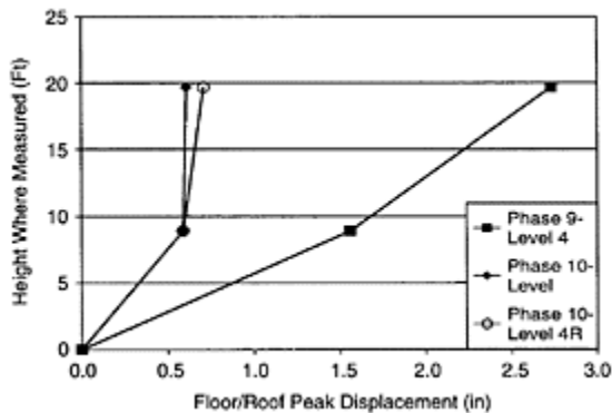
FIGURE 18.21 Vertical distribution of deformation demand in UC San Diego House. (From Cobein et al., 2003, CUREE Publication W-30, CUREE, Richmond, CA. With permission.)
