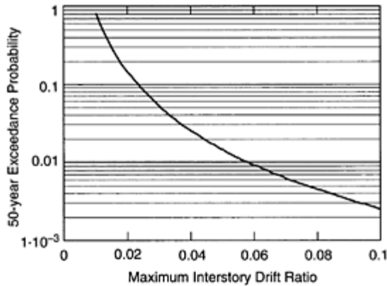
FIGURE 7.3 Fifty-year maximum interstory drift ratio demand curve.
