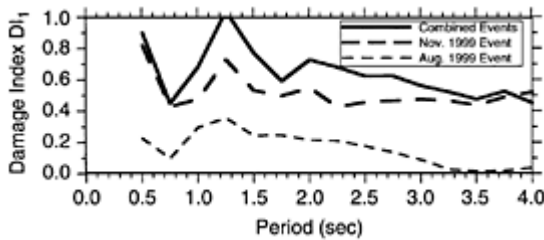
FIGURE 5.21 Damage spectra for the individual ground motions recorded at Düzce (EW component) during the August 17, 1999 Kocaeli and November 12, 1999 Düzce earthquakes in Turkey and for the combined ground motion time histories (see also Figure 5.16(a)).
