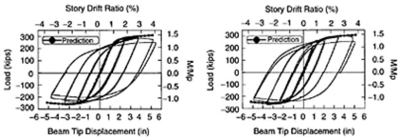
FIGURE 15.16 Load versus beam tip deflection relationships of the composite specimen (Yu, Q.-S., Noel, S. and Uang, C.-M. (1997). Experimental studies on seismic rehabilitation of pre-Northridge steel moment connections: RBS and haunch approach, Report No. SSRP-97/08, University of California, San Diego, CA).
