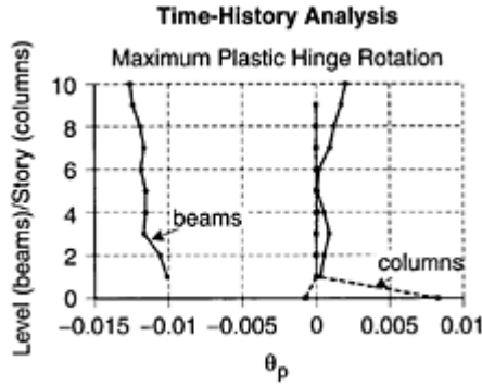
FIGURE 8.53 Maximum plastic hinge rotations for time-history analysis.
