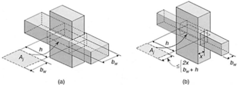
FIGURE 14.36 Definition of A_j for joint shear determination.
