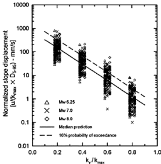
FIGURE 4.46 Normalized sliding displacement (Modified from Bray, J.D. and Rathje, E.M. (1998). J.
