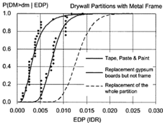
FIGURE 9.41 Fragility functions for three damage states of drywall partitions with metal frames.
