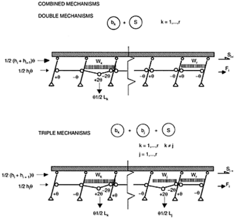
FIGURE 8.10 Combined mechanisms.
