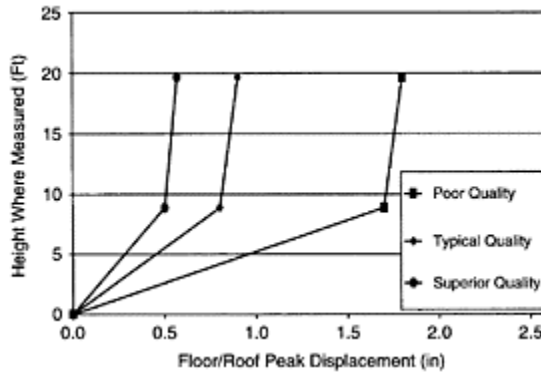
FIGURE 18.22 Vertical distribution of deformation demand in Large House Index Building considering three levels of construction quality. (From Cobeen et al., 2003, CUREE Publication W-30, CUREE, Richmond, CA. With permission.)
