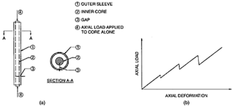
FIGURE 16.22 Concept of sleeved column and typical behavior, (a) Components of sleeved column; (b) typical compression behavior.
