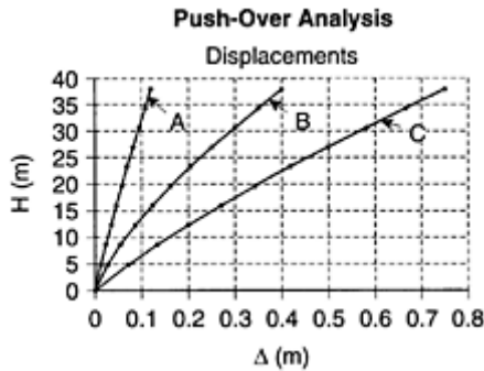
FIGURE 8.45 Displacements for push-over analysis.
