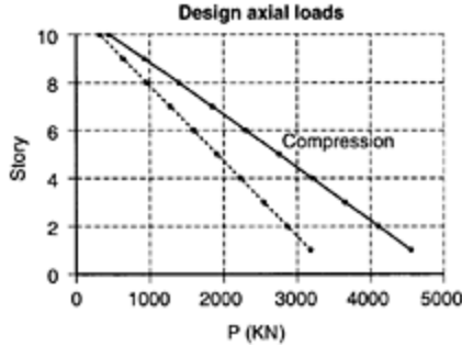
FIGURE 8.33 Design axial load for interior column.
