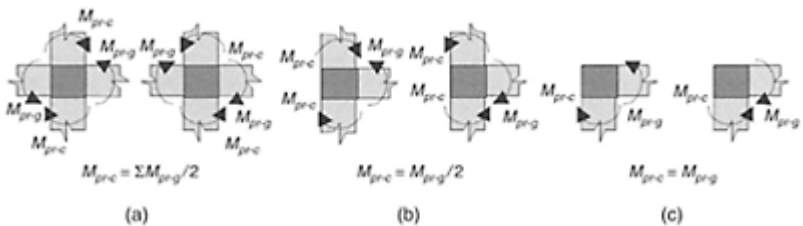
FIGURE 14.34 Maximum M_{pr} for the columns needed to obtain column shear V_e .
