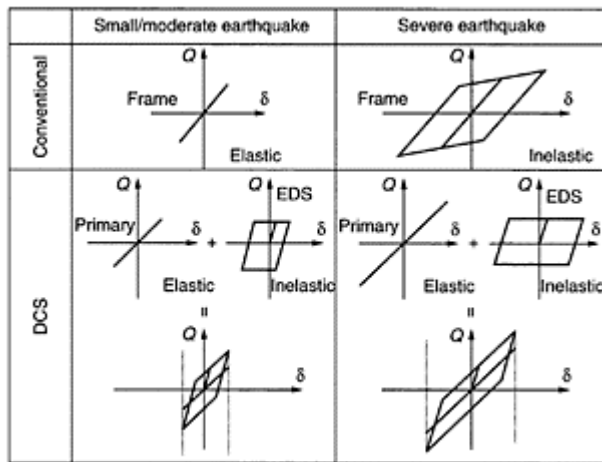
FIGURE 10.9 Structure with energy dissipating system.
