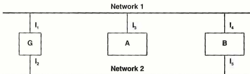
Figure 4.2 An example internet with a multi-homed host, B, that demonstrates a problem with the IP addressing scheme. If interface I_4 becomes disconnected, A must use address I_5 to reach B, routing packets through gateway G.
