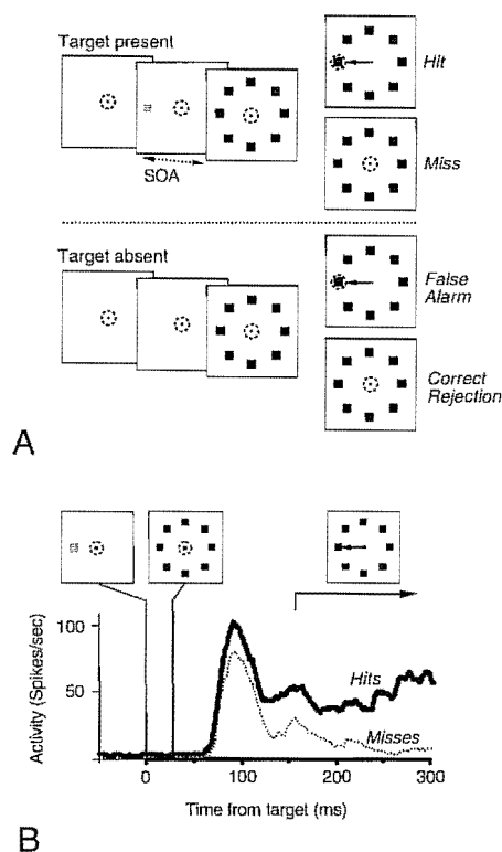
FIGURE 9.7 Response of FEF to a masked target. (A) Visual backward masking task. The target appeared followed after an adjustable stimulus onset asynchrony (SOA) by a mask in target-present trials. A saccade directly to the location where the target had been was scored a Hit . Continued fixation was scored a Miss . Only the mask appeared on target-absent trials. A saccade to any location was scored a False Alarm . Continued fixation was scored a Correct Rejection . Monkeys were rewarded for hits and correct rejections. (B) Activity of a FEF visual neuron. The panel compares the activity during target-present trials leading to hits (thick) and misses (thin). Trials are aligned on the time of target presentation in the left panels and on time of mask presentation in the right panels. The differences between alternative trials are shown in the bottom panels. (Modified from Reference 89.)
