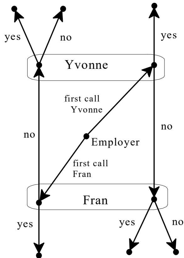
Figure 4.4: The extensive form, or frame, representing Example 4.2
