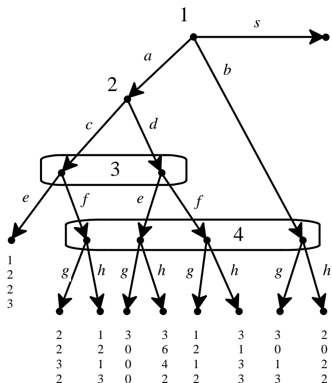
Figure 13.16: The game for Exercise 13.6.
