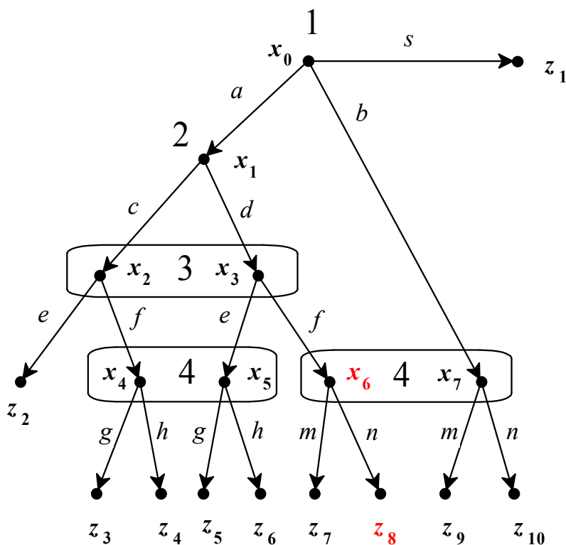
Figure 13.1: A game-frame in extensive form.
