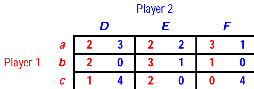
Figure 2.53: The game for Exercise 2.21
