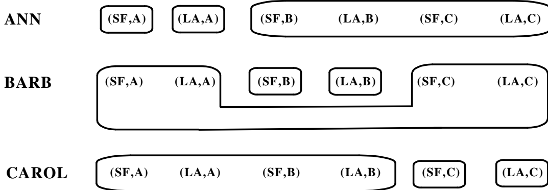
Figure 8.19: The information partitions for Exercise 8.7.
