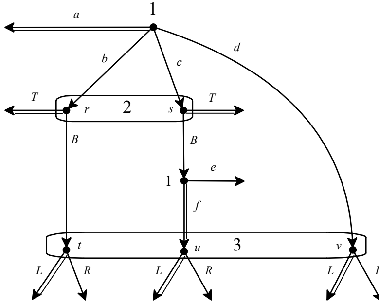
Figure 12.3: The assessment \sigma = (a, T, f, L) , \mu(r) = \mu(s) = \frac{1}{2} , \mu(t) = \frac{1}{5} , \mu(u) = \mu(v) = \frac{2}{5} is not consistent.
