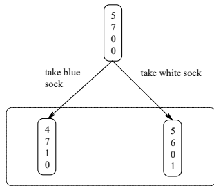
Figure 8.16: The possible states after taking one sock.
