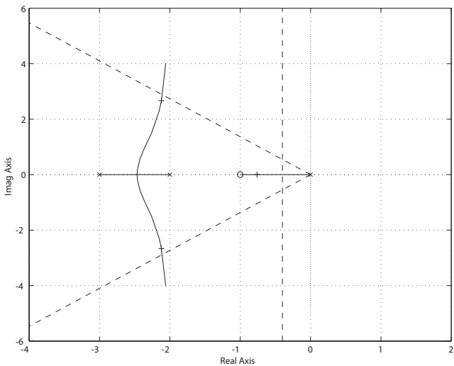
FIGURE CP7.7 CONTINUED: (d) Root locus for PI controller with selected K = 9.2516 .
