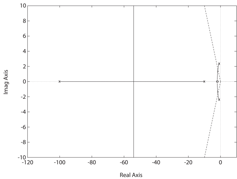
FIGURE P7.10 Root locus for 1 + \frac{K_1 K_2 (s + 2)^2}{(s + 10)(s + 100)(s^2 + 1.5s + 6.25)} = 0 .
