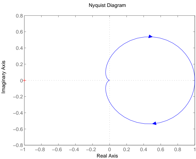
FIGURE P8.1 (a) Polar plot for G_c(s)G(s) = \frac{1}{(1+0.25s)(1+3s)} .
