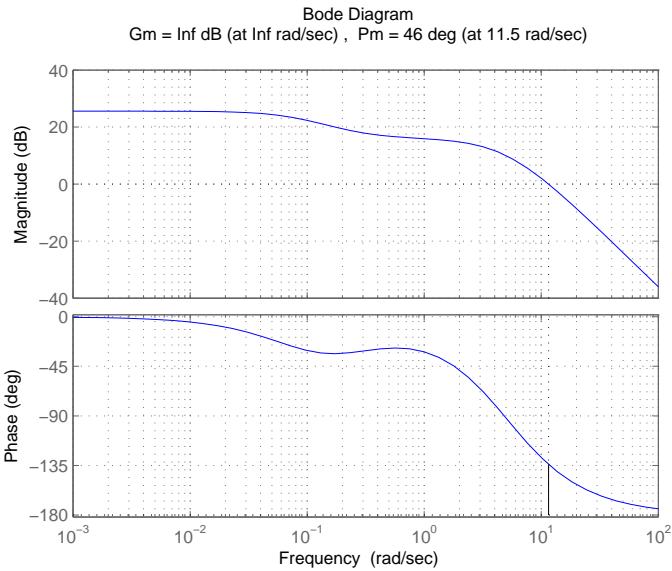
FIGURE P10.23 Bode plot for G_c(s)G(s) = \frac{475(4s+1)}{(s+5)^2(12s+1)} .
