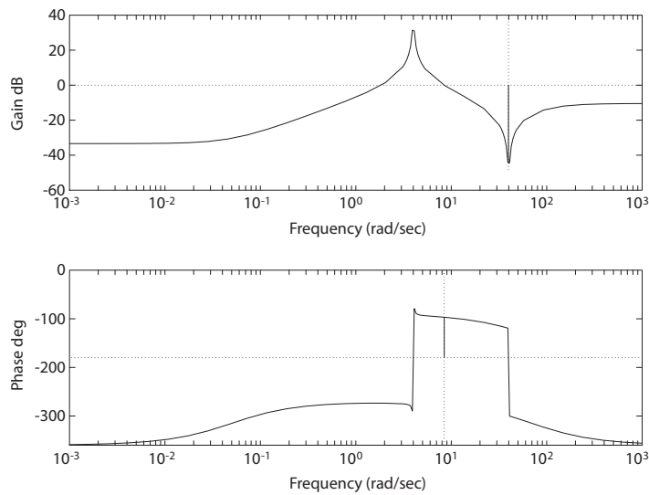
FIGURE P9.9 (a) Bode Diagram for G_c(s)G(s)H(s) = \frac{0.3(s+0.05)(s^2+1600)}{(s+70)(s^2+0.05s+16)} .
