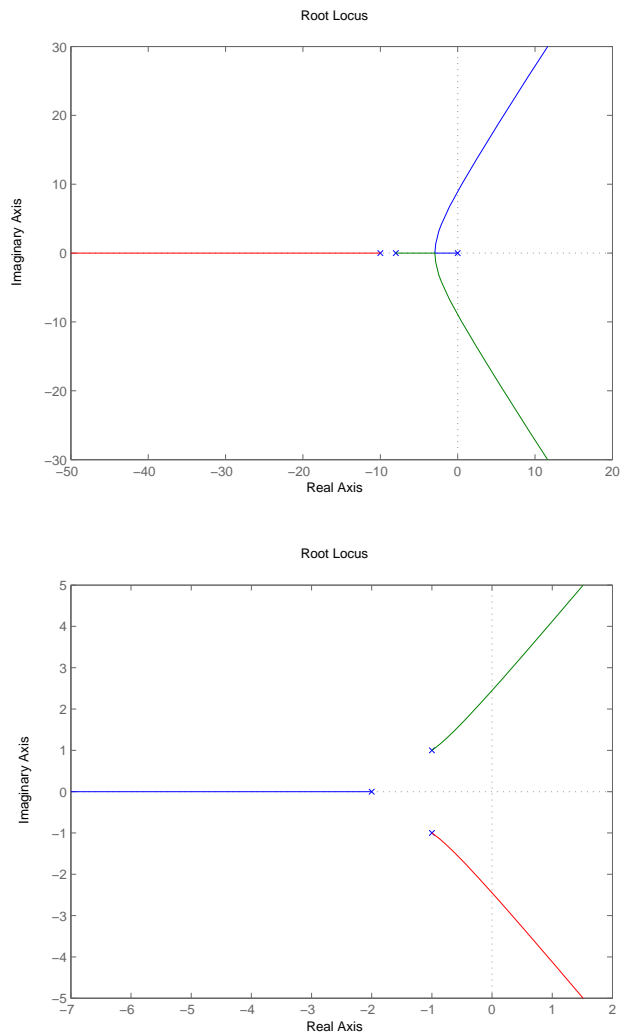
FIGURE P7.1 (a) Root locus for 1 + \frac{K}{s(s+10)(s+8)} = 0 , and (b) 1 + \frac{K}{(s^2+2s+2)(s+1)} = 0 .
