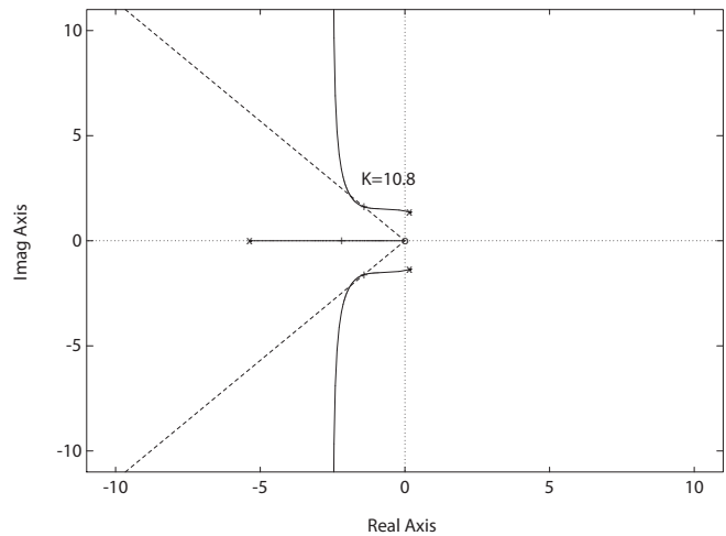
FIGURE E7.21 Root locus for 1 + \frac{Ks}{s^3 + 5s^2 + 10} = 0 .
