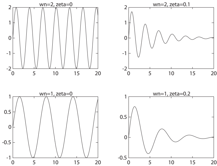
FIGURE CP5.3 Impulse responses.
