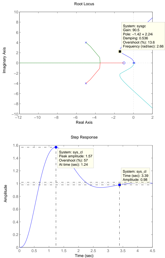
FIGURE DP7.5 (a) Root locus for 1 + K \frac{s+1}{s(s-0.1)(s^2+10s+41)} = 0 . (b) Step response with K = 875 .
