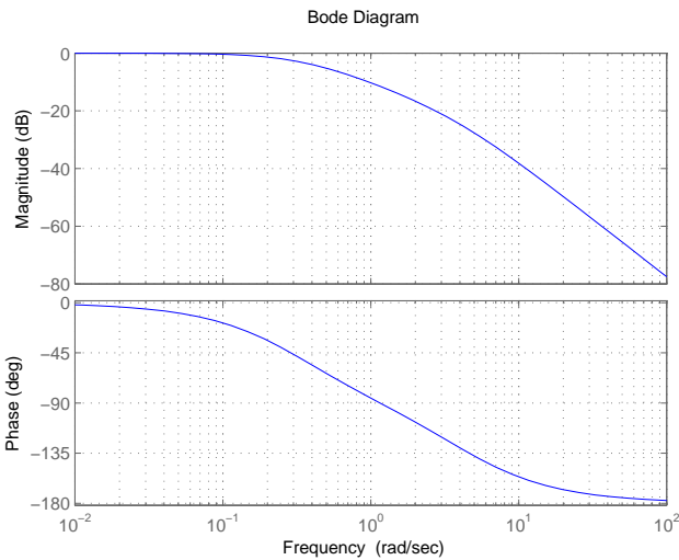
FIGURE P8.2 (a) Bode plot for G_c(s)G(s) = \frac{1}{(1+0.25s)(1+3s)} .
