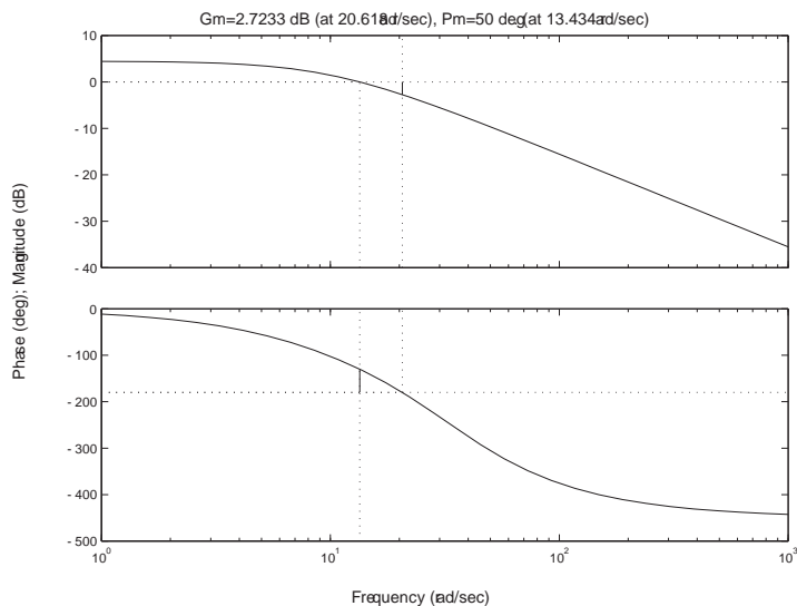
FIGURE E9.19 Bode Diagram for G_c(s)G(s) = K \frac{e^{-0.1s}}{s+10} , where K = 16.75 .
