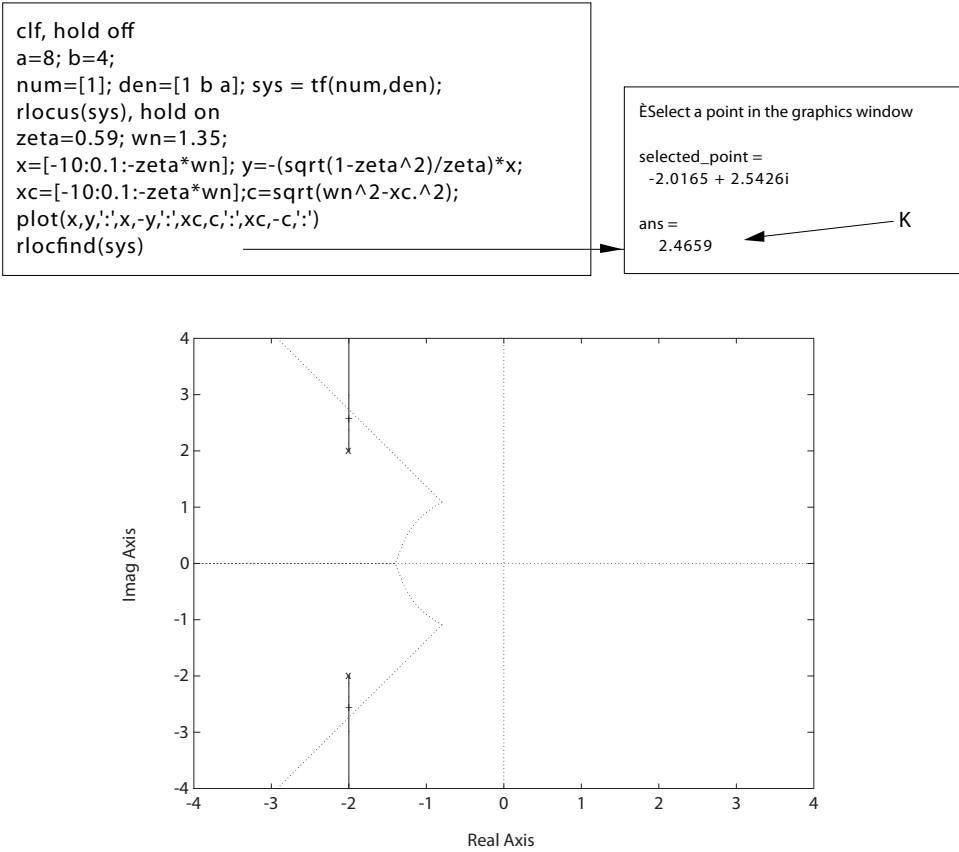
FIGURE CP12.4 (a) Root locus for 1 + K \frac{1}{s^2 + 4s + 8} .
