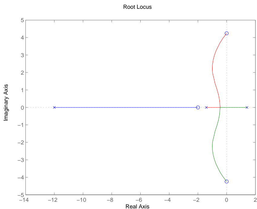
FIGURE E7.22 Root locus for 1 + \frac{K(s^2 + 18)(s + 2)}{(s^2 - 2)(s + 12)} = 0 .
