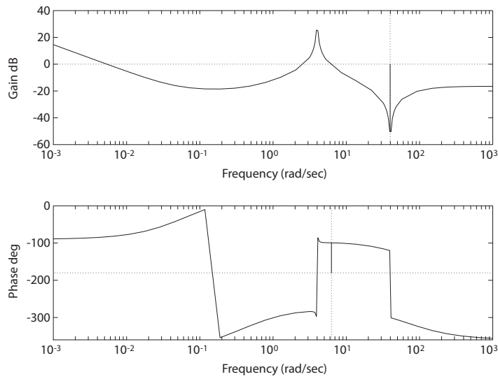
FIGURE P9.9 CONTINUED: (b) Bode Diagram for G_s(s)G(s)H(s) = \frac{0.15K_1(s+0.05)(s^2+1600)(s+0.5)}{(s+70)(s^2+0.05s+16)} , K_1 = 1 .
