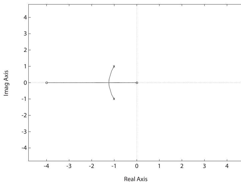
FIGURE E7.1 Root locus for 1 + K \frac{s(s+4)}{s^2 + 2s + 2} = 0 .
