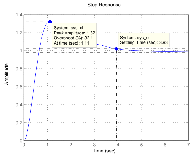
FIGURE DP8.7 Step response for K_P = 5.5 , K_I = 3.33 , and K_D = 3.5 .
