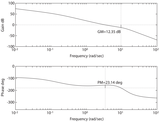
FIGURE E9.10 (a) Bode Diagram for G_c(s)G(s) = \frac{326s+1304}{s^4+14.76s^3+151.3s^2+23.84s} .
