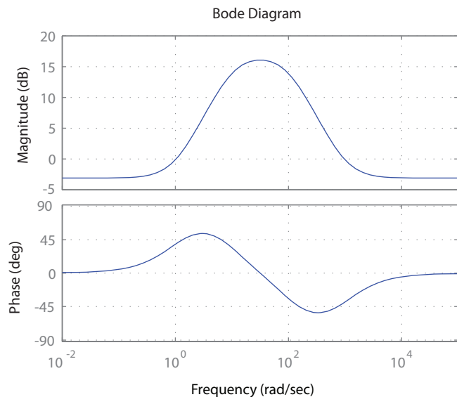
FIGURE CP8.9 Bode plot for G(s) = 0.7 \frac{(s+1000)(s+1)}{(s+100)(s+10)}
