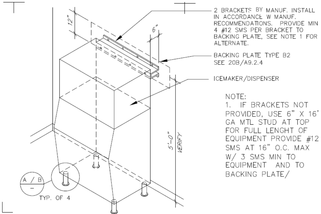
37 ICEMAKER/DISP AND SIMILAR ANCHORAGE (COORD WITH MANUFACTURER) SCALE: NO SCALE
