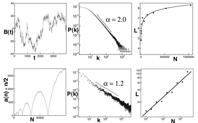
Fig. 4. Fractal series. (Upper from left to right) First 4,000 data values from a Brownian series of 10^6 data values. (Center) The degree distribution of the visibility graph associated with the Brownian motion. This one is a power law P(k) \sim k^{-\alpha} with \alpha = 2.00 \pm 0.01 . (Right) Plot of the mean path length of this network as a function of the network size N . The best fitting provides a logarithmic scaling L(N) = 1.21 + 0.51 \log(N) . This network shows small-world effect in addition to being scale-free. (Lower from left to right) First 10^5 data values from a Conway series of 4 \cdot 10^6 data values. (Center) The degree distribution of the visibility graph associated with the Conway series. This one is a power law P(k) \sim k^{-\alpha} with \alpha = 1.2 \pm 0.1 . The mean path length as a function of the size N is depicted in Right. The best fitting provides a power law scaling L(N) = 0.76N^{0.38} . Then, this network is scale-invariant.
