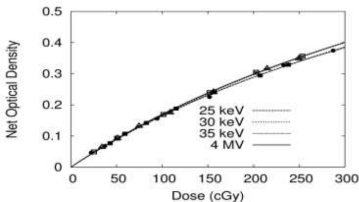
Fig 7: Net optical density versus dose for EBT3 film. The film was calibrated at 25 keV (circles), 30keV (triangles), 35 keV (filled squares) and 4 MV (hollow squares). Each set of data were fitted with the function shown in Eq. (2). [12]
