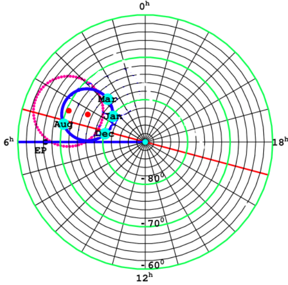
Figure 4: South celestial pole region. The dot (red) at RA=4.3 h , Dec=75°S, and with speed 486km/s, is the direction of motion of the solar system through space determined from NASA spacecraft Earth-flyby Doppler shifts [6], as revealed by the EM radiation speed anisotropy. The thick (blue) circle centred on this direction is the observed velocity direction for different months of the year, caused by Earth orbital motion and sun 3-space inflow. The corresponding results from the 1925/26 Miller gas-mode interferometer are shown by 2nd dot (red) and its aberration circle (red dots). For December 8, 1992, the speed is 491km/s from direction RA=5.2 h , Dec=80°S, see Table 2 of [6]. EP is the pole direction of the plane of the ecliptic, and so the space flow is close to being perpendicular to the plane of the ecliptic.
