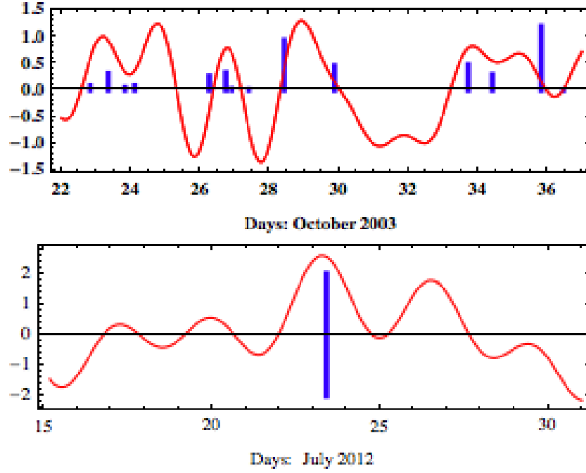
Figure 6: Top: Vertical blue lines indicate start times of major solar flares beginning October 22, 2003. The height of the lines is indicative of the magnitude of the solar flare, and is on a logarithmic scale. These solar flares are known as the Halloween Space Weather Storms of 2003, [12]. The curve is data from a single ZDQD, located in Switzerland, low-pass filtered to include only periods longer than 2 days, and advanced in time by 6 days, and plotted relative to the average. For a space speed of 500km/s this corresponds to a cell size \sim 0.5 of the Sun-Earth distance. This advance followed from matching the two data sets. The low-pass filter ensures that we see space fluctuations corresponding to cell sizes that can overlap the Earth and the sun, as the space flow is close to being perpendicular to the plane of the ecliptic, as shown by the analysis of the NASA Earth-flyby spacecraft Doppler shifts in Fig.4, [6]. The strong correlation between the two data sets show that solar flares follow increases in the space velocity, by some 6 days: the solar flares are caused by the space fluctuations: these fluctuations are a galactic phenomenon. Bottom: Vertical blue line indicates start of massive Coronal Mass Ejection (CME) on July 23, 2012, and plotted with ZDQD low-pass data, but without time shift. The main speed fluctuation peak coincides with the CME, on July 23. This suggests that CME may not be caused by space fluctuations, and that the coincident peak may be gravitational waves produced by the extremely large mass ejection, although there is a smaller peak in the ZDQD data some 6 days earlier.
