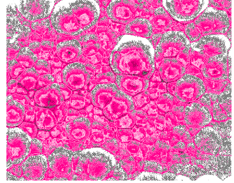
Figure 5: Representation of the fractal wave data revealing the fractal textured structure of the 3-space, with cells of space having slightly different velocities and continually changing, and moving wrt the Earth with a speed of ~500 km/s, and in the directions indicated in Fig.4, namely almost perpendicular to the plane of the ecliptic. This “red space” is suggestive of the 1/f spectrum of the detected fluctuations, see [5]. These space flow fluctuations inject energy into both the sun and the Earth. For solar flare effects low pass filtering of the data is necessary to isolate cells that overlap the Earth and sun, as in Fig.6.
