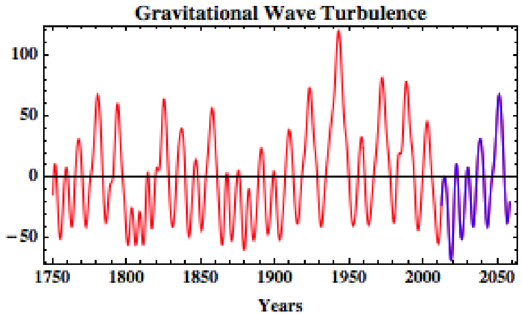
Figure 7: Plot of Gravitational Wave Turbulence vs years 1749 to present (red plot), based upon Solar Flare counts as a proxy, as shown in Fig. 1. Data adapted from from D. Archibald, Solar Update March 2012 ( http://www.warwickhughes.com/blog/?p=2753 ), [15]. The Solar Flare data has been low-pass filtered using Fast Fourier Transforms. It is argued herein that the 11 year cycle and longer cycles are caused by galactic space flow turbulence, which can now be easily measured using ZDQD. Beyond 2014 we have used the Fourier amplitudes to extrapolate to 2050 (blue plot), which assumes an ongoing 1/f spectrum. This extrapolation suggests we are facing an epoch of low space flow turbulence, and hence reduced Earth temperatures. The modern warm period extended from 1900s to end of solar cycle 23 (the last cycle in red).
