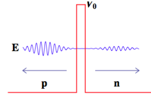
Figure 3: Reflected (LHS) and transmitted (RHS) wave packets after interaction with barrier at a reverse-biased pn junction, as in Fig.2. Energy E of wave packet is less than potential barrier height V_0 . The wave function transmission varies with the speed v of the passing space as that varies E \rightarrow E + \hbar k \cdot v according to (1) and so we may measure v .
