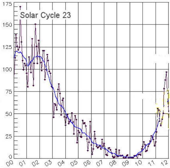
Figure 1: Top: Measure of Zener diode GCP network current fluctuations over Solar Cycle 23, beginning with zero on January 1, 2000, adapted from R. Nelson, Long Term Cumulative Deviation of Network Variance : http://noosphere.princeton.edu/longterm.html . Bottom: Sunspot numbers for the same time period, adapted from T. Phillips, http://science.nasa.gov/media/medialibrary/2013/03/01/shortfall.jpg . We see the close correlation between these two phenomena. A causal relationship between space speed fluctuations and sunspots is demonstrated in Fig.6: space flow fluctuations/turbulence precede by some 6 days the solar flares, implying that it is the space flow turbulence that causes the solar flares. This data shows the weakening of the solar cycle as being caused by weakening of the space flow turbulence. The data in Fig.8 shows sea temperature history tracking solar flares, but not caused by the solar flares. There is a fundamental difference between correlations and cause and effect dynamics.
