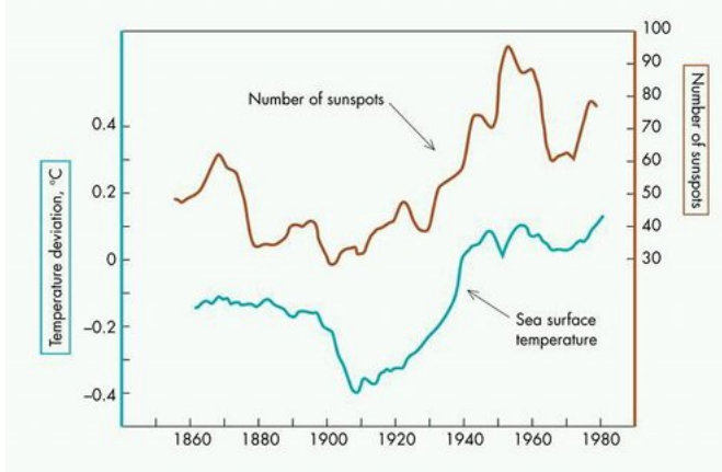
Figure 8: Shows strong correlations between solar sunspot numbers and Earth sea surface temperature deviations. This, however, does not imply a causal relation between these two phenomena, as was also noted in Fig.1. It is conjectured herein that the cause is the galactic space flow turbulence, which pumps energy into both the sun and the Earth.
