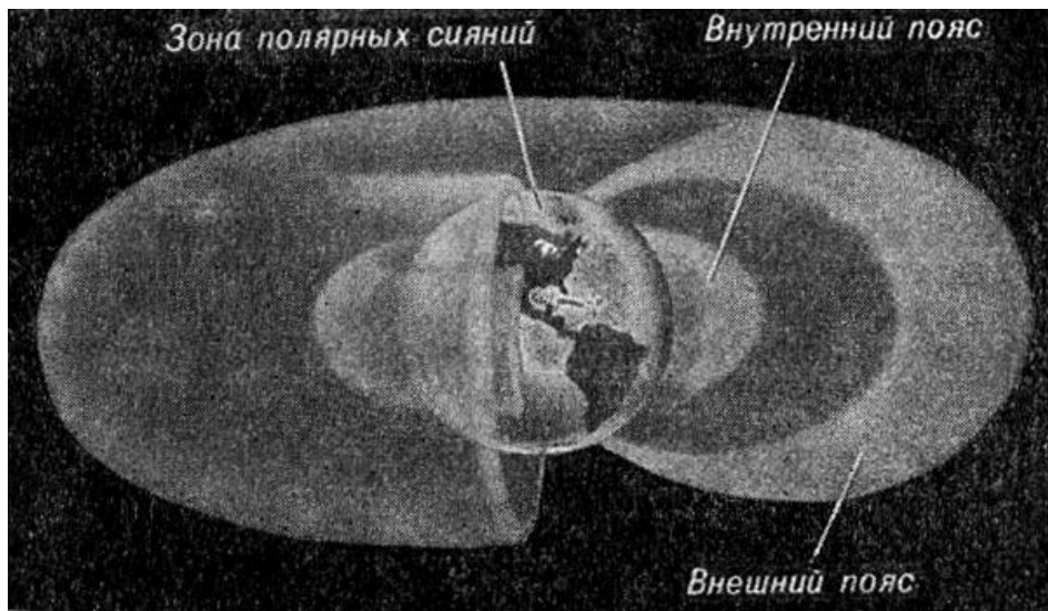
Fig 4. Earth's Radiation Belt
