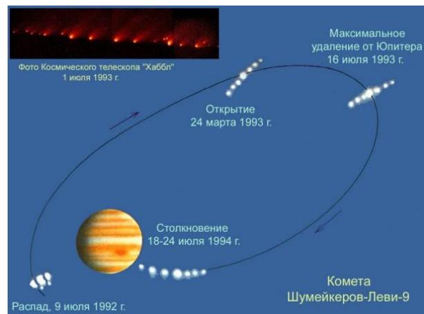
Fig. 2. The orientation of the fragments of Comet Shoemakerov-Levy-9
