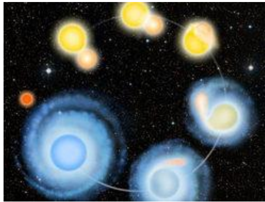
Fig. 3. Polarization of a cluster of galaxies
