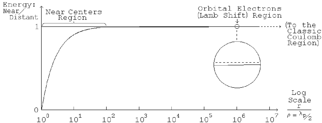
Figure 3 Coulomb Effect Reduction Factor When Charges Are Near to Each Other
