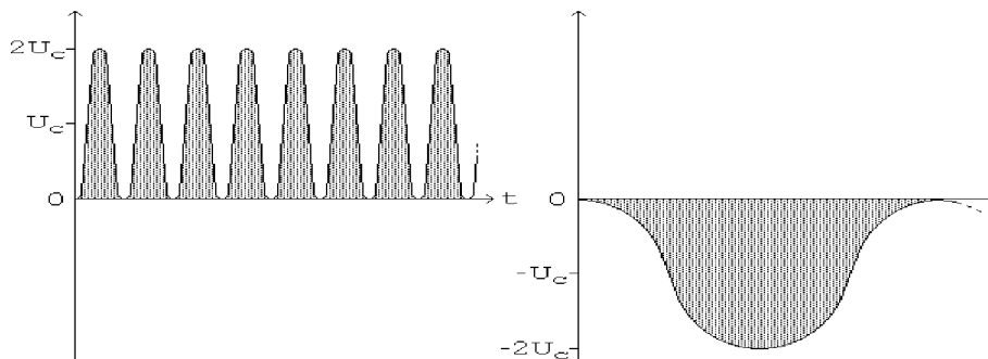
Figure 1(a) Oscillations at Two Different Frequencies
