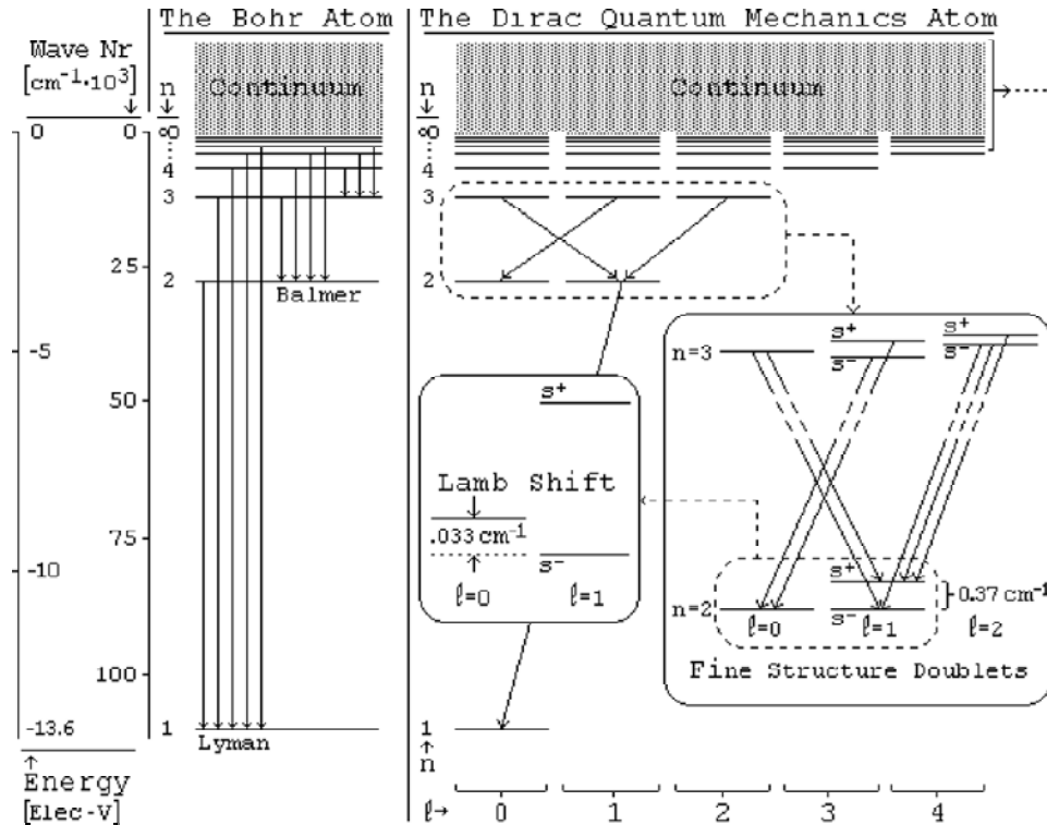
Figure 4 Hydrogen Spectra and the Lamb Shift
