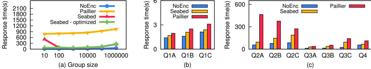
Figure 9: (a) Microbenchmark results for group-by queries. (b-c) Response time for the Big Data Benchmark queries.
