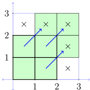
Figure 20: The boundary strip for a 3 \times 3 square contains 5 tiles, which is 2 more than the previous boundary strip.
