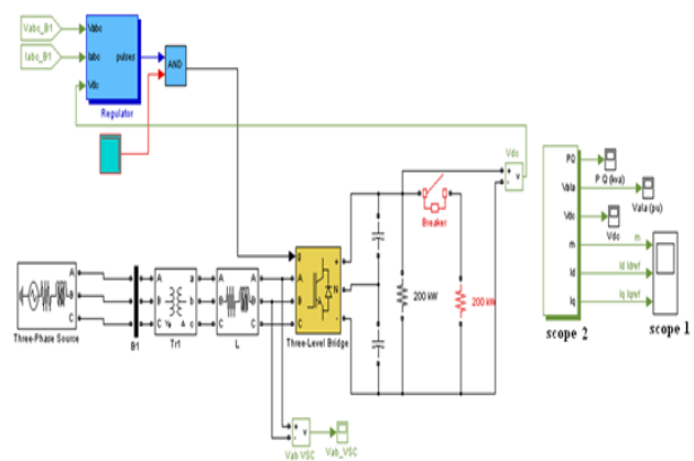
Figure 4: proposed converter using a three-phase three-level PWM Voltage-sourced Converter
