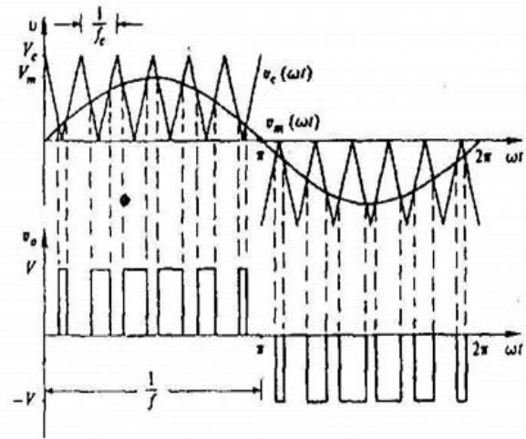
Fig (1) Reference and timing wave forms for unipolar pulse width modulated control signal
