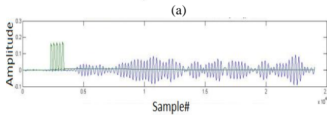
Fig. 3. (a) Signal from structure with flaw (b) Signal from structure without flaw
