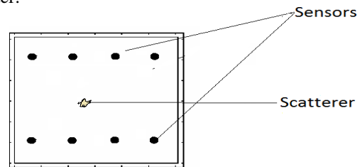
Fig. 2 Position of sensors on the plate
