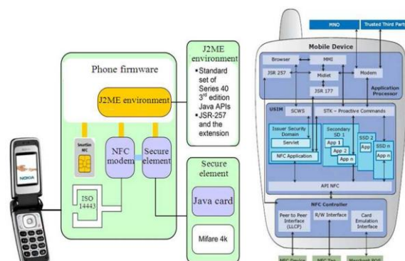
a) Architecture of NFC technology in a mobile device defined by NFCF in 2011 and (b) NFC integrated inGSM A (2011)
