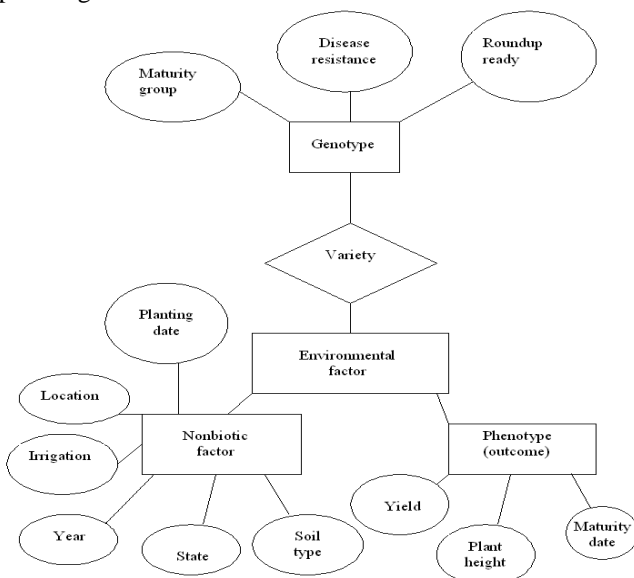
Figure.4 a model of agriculture agronomy
