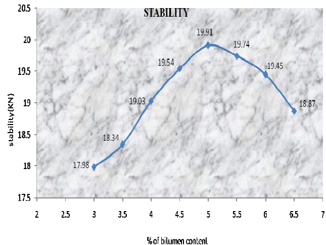
Fig No-4 Stability (KN) V/s % of bitumen content for 5% plastic mix
