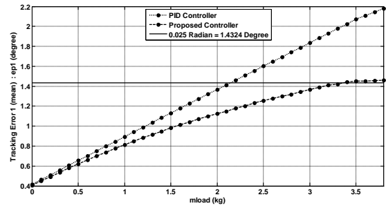
Fig 3. Comparison between conventional PID controller and proposed controller in determining of maximum load carrying capacity (tracking control case).
