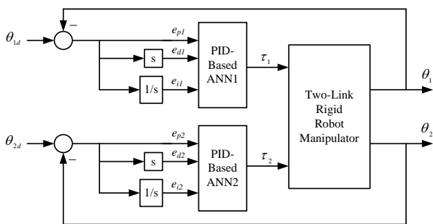
Fig 1. Block diagram of the two rigid-link robot manipulator control system.
