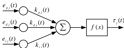
Fig 2. Block diagram of a nonlinear PID-based neural network.
