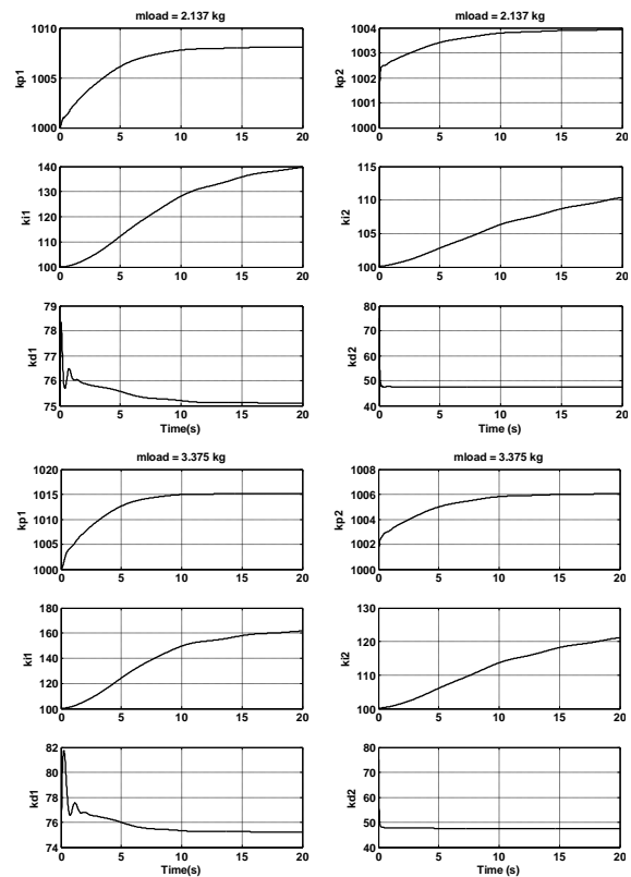
Fig 6. Updating of each control parameter ( k_p , k_i and k_d ).
