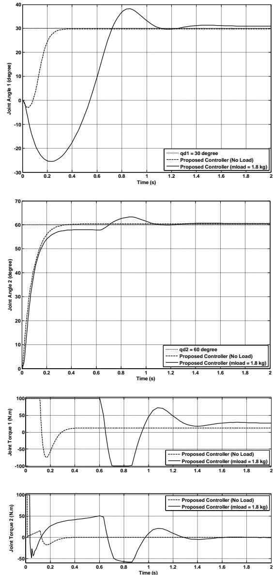
Fig 9. Results of proposed nonlinear PID controller using neural network in two no load and maximum load ( m_{load} = 1.8^{kg} ) cases.
