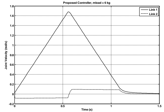
Fig 11. Links velocity.
