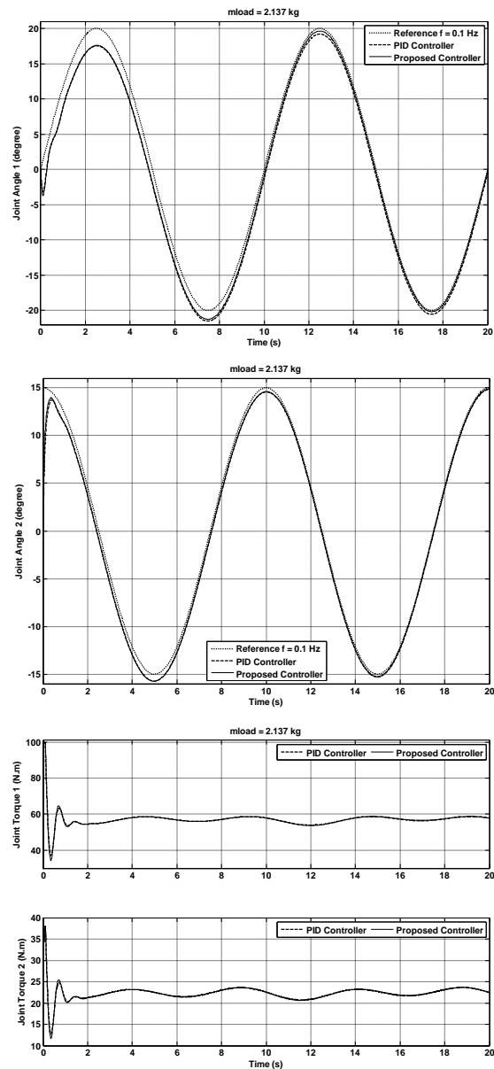
Fig 4. Comparison between conventional PID controller and nonlinear PID controller using neural network (frequency of reference f = 0.1^{Hz} and m_{load} = 2.137^{kg} ).
