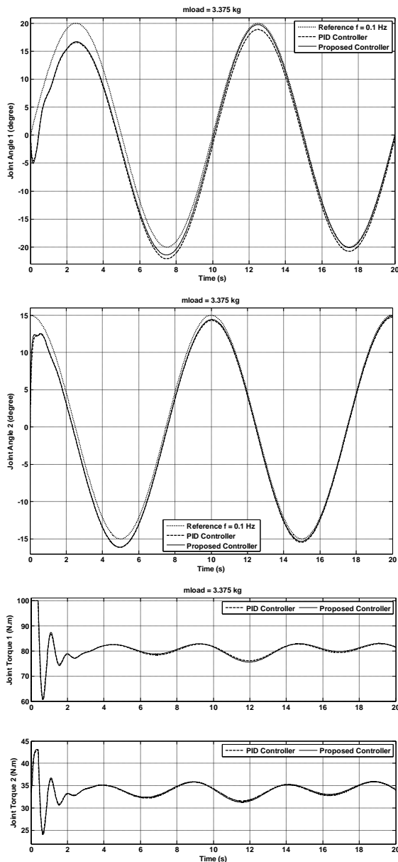
Fig 5. Comparison between conventional PID controller and nonlinear PID controller using neural network (frequency of reference f = 0.1\text{Hz} and m_{load} = 3.375\text{kg} ).
