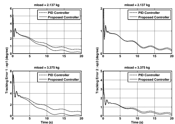
Fig 7. Comparison tracking error between conventional PID controller and proposed controller.
