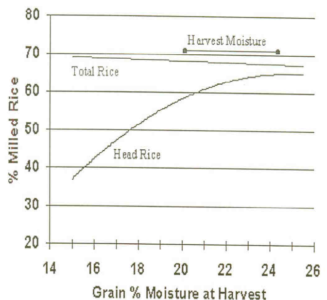
Figure 1. Effect of Grain Moisture Content at Harvest on Milling and Head Rice Recovery
