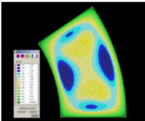
a) The vertical displacements of the shell on four unmovable linear hinges ( W_{\max} = 2,53 mm)
