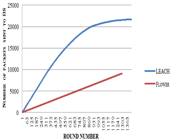
Figure 2. Number of packets sent to BS vs. round using LEACH vs. FPOA.
