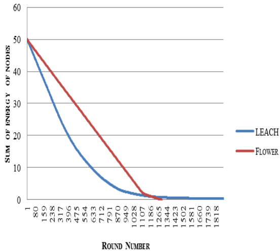
Figure 5. Sum of energy of nodes vs. round using LEACH vs. FPOA.
