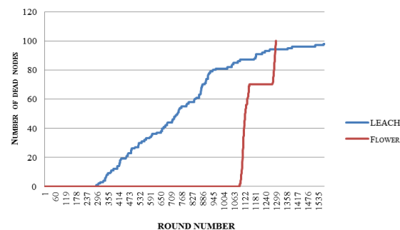
Figure 4. Number of dead nodes vs. round using LEACH vs. FPOA.
