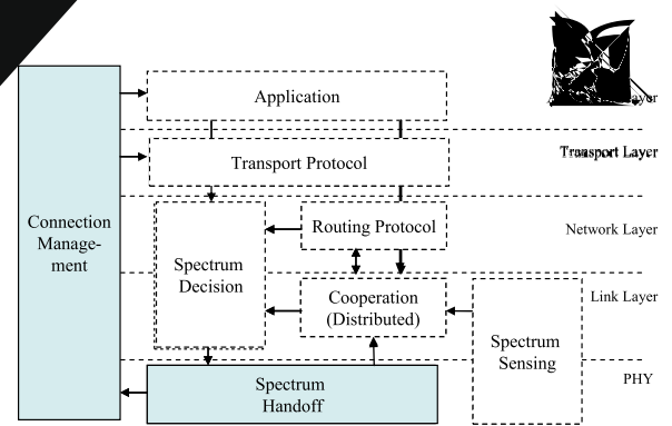
Fig. 16. Spectrum mobility structure for ad hoc CR networks.
