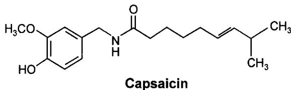
Fig. 8.1 Chemical structure of capsaicin.
