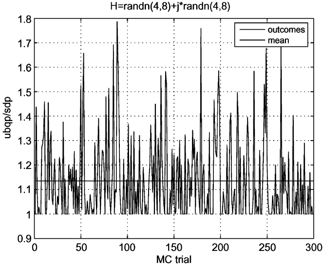
Fig. 3. Upper bound on v_{qp}/v_{sdp} for m = 8 , n = 4 , over 300 realizations of complex Gaussian i.i.d. channel vector entries.
