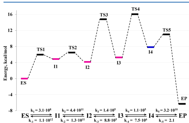
Figure 4. Energy profile for the GTP hydrolysis at the active site of the Ras-GAP complex. The bottom panel shows values of the monomolecular reaction rate constants k_{in} and k_{-n} (in s^{-1} ) estimated by using the transition state theory for every elementary step on the route.
