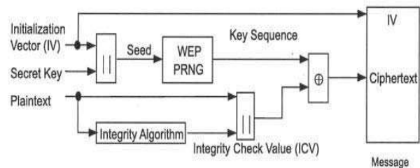
Figure shows the encryption process of WEP.
