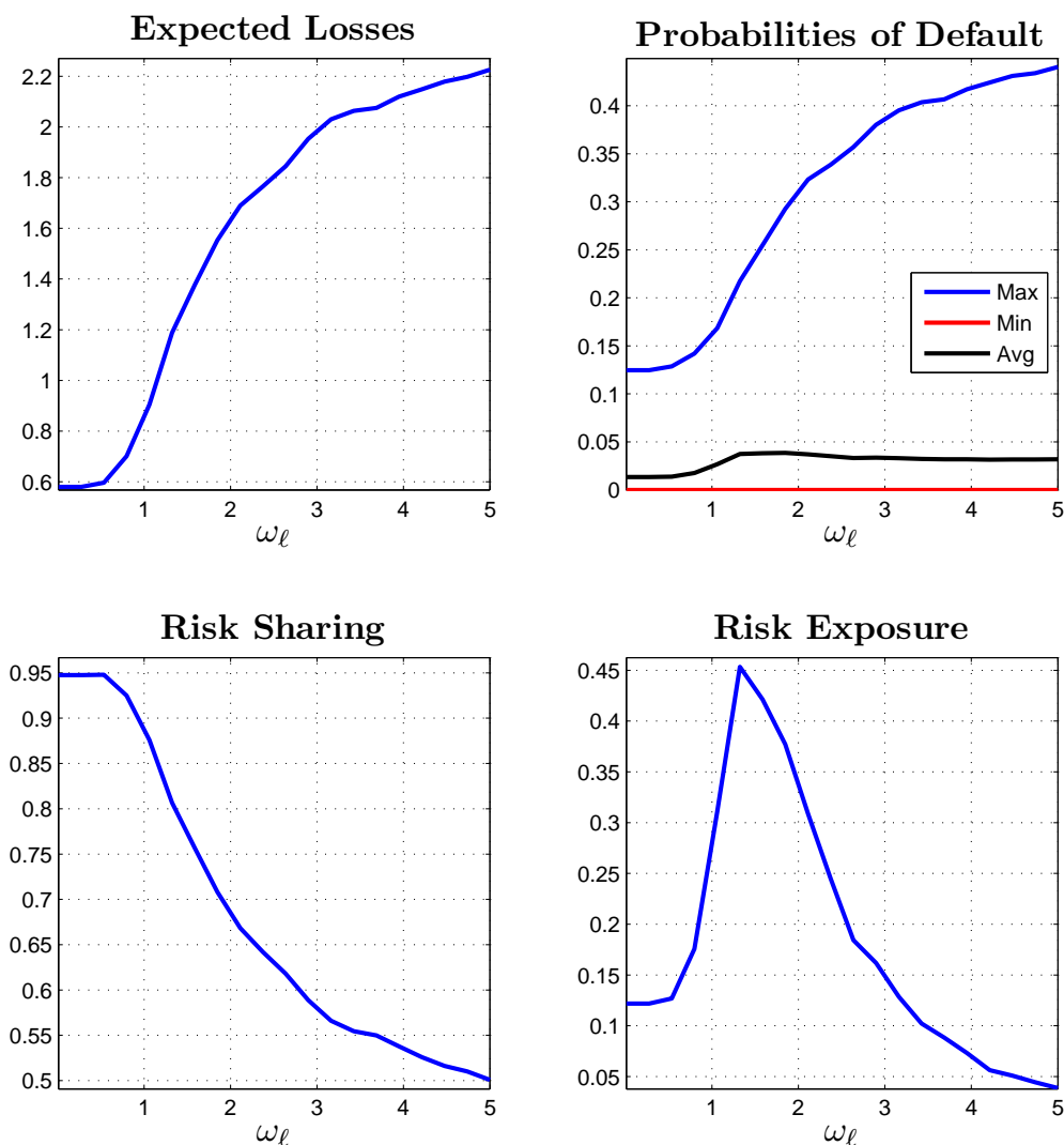
Figure 12: Changes in \omega_\ell
