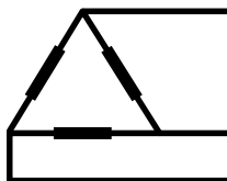
Figure 1.2 – Three phase delta, three wire
