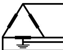
Figure 1.5 – Three phase delta, four wire, grounded neutral
