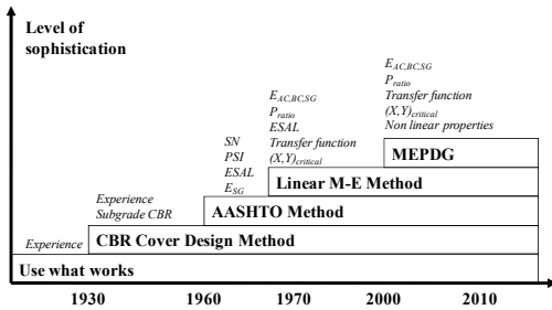
Figure 5: Evolution of pavement design methods (Reck 2009)
