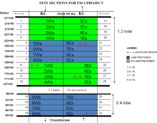
Figure 12: Schematic layout of test sections at FM 2 site (Gupta et al. 2008)
