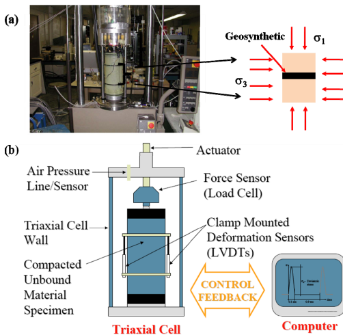
Figure 18: Cyclic triaxial test (a) Test equipment (Perkins et al. 2004); (b) Schematic of test setup (Tutumluer 2004)
