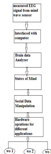
Figure 3: Flow chart for Brain Data Analyzer system.
