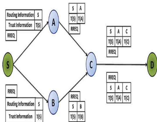
Figure 8 Trust value propagation through RREQ packets
