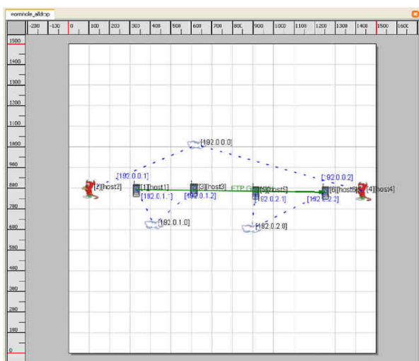
Figure 6 Wormhole attack model
