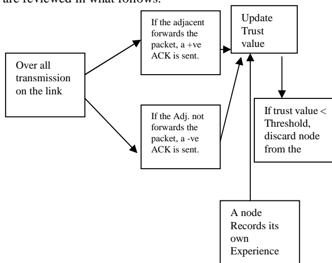
Figure 3 Functions of Trust models
