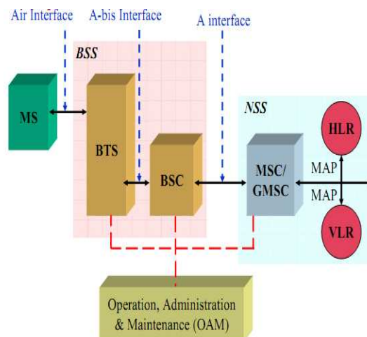
Figure 1: GSM Network Architecture
