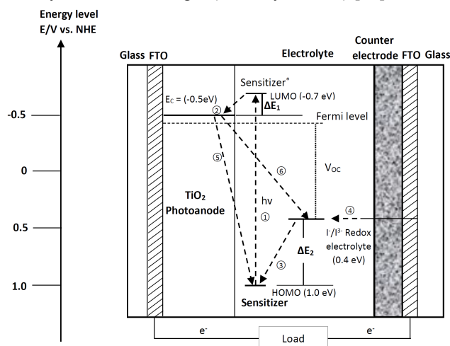
Fig. 1. Schematic energy diagram and operating principle of DSSC. Adapted from [Source: 13].
