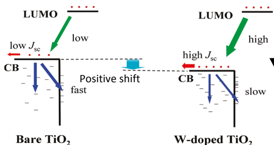
Fig. 2. Positive shift in E c of TiO 2 with W doping increases the driving force for electron injection (increases in J sc ) and suppress recombination [Source:75].
