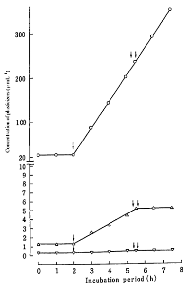
Figure 3: Changes of the concentrations of PA, MEHP, and DEHP when incubated at 37 °C: (a) without addition of enzymes to plasma (○=DEHP, △=MEHP, ▽=PA); (b) with addition of lipase (3.6mg/ mL, 100 µL) or esterase (10 mg/mL, 100 µL) ti okasna (○=DEHP, △=MEHP, ▽=PA); (c) with addition of lipase (3.6mg/mL, 278 µL; (○=DEHP, △=MEHP, ▽=PA) or esterase (10 mg/mL, 100 µL; ●=DEHP, ▲=MEHP, ▼PA) to plasma.
