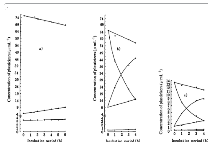
Figure 2: Changes of the concentrations of PA, MEHP, and DEHP when incubated at 37 °C: (a) without addition of enzymes to plasma ( \circ =DEHP, \Delta =MEHP, \nabla =PA); (b) with addition of lipase (3.6mg/ mL, 100 \mu\text{L} ) or esterase (10 mg/mL, 100 \mu\text{L} ) to plasma ( \circ =DEHP, \Delta =MEHP, \nabla =PA); (c) with addition of lipase (3.6mg/mL, 278 \mu\text{L} ; \circ =DEHP, \Delta =MEHP, \nabla =PA) or esterase (10 mg/mL, 100 \mu\text{L} ; \bullet =DEHP, \blacktriangle =MEHP, \blacktriangledown =PA) to plasma.
