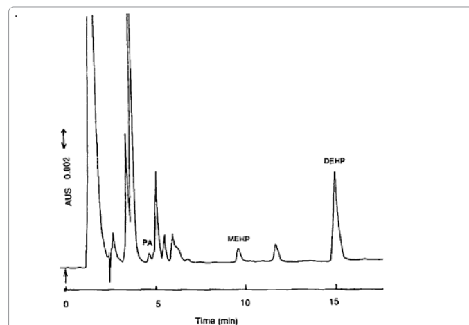
Figure 1: HPLC chromatogram obtained after SPE of fresh frozen human plasma from the Japanese Red Cross. Recovery of PA from plasma was somewhat unsatisfactory, because of the hydrophilicity of the compound; recovery was, however, sufficient for quantitative work, as mentioned in the text.
